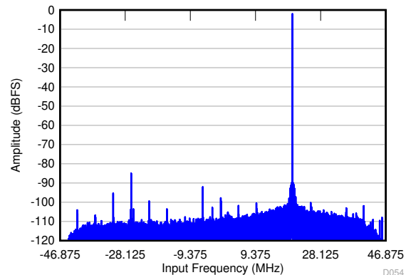
f_{IN} = 1.78 \text{ GHz} , A_{IN} = -2 \text{ dBFS} , f_S = 2949.12 \text{ MSPS} , SNR = 64.5 dBFS, SFDR (includes IL) = 79 dBc
