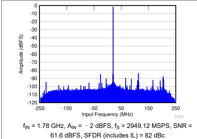
图 6-69. FFT in 6x Decimation (Complex Output)
