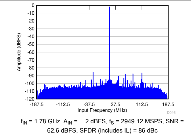
图 6-70. FFT in 8x Decimation (Complex Output)
