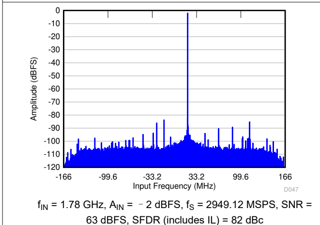
图 6-71. FFT in 9x Decimation (Complex Output)
