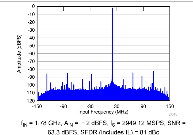
图 6-72. FFT in 10x Decimation (Complex Output)
