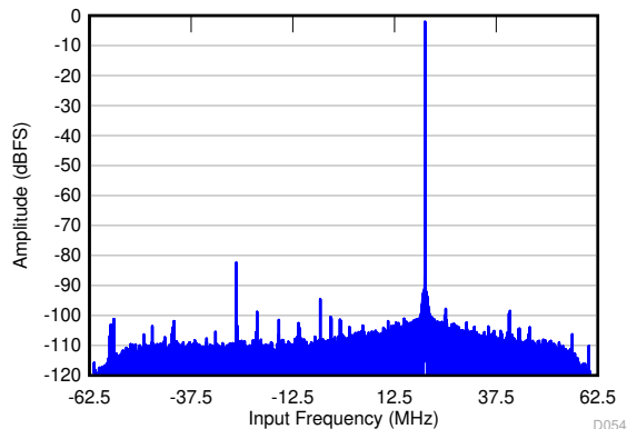
f_{IN} = 1.78 \text{ GHz} , A_{IN} = -2 \text{ dBFS} , f_S = 2949.12 \text{ MSPS} , SNR = 64.4 dBFS, SFDR (includes IL) = 82 dBc
