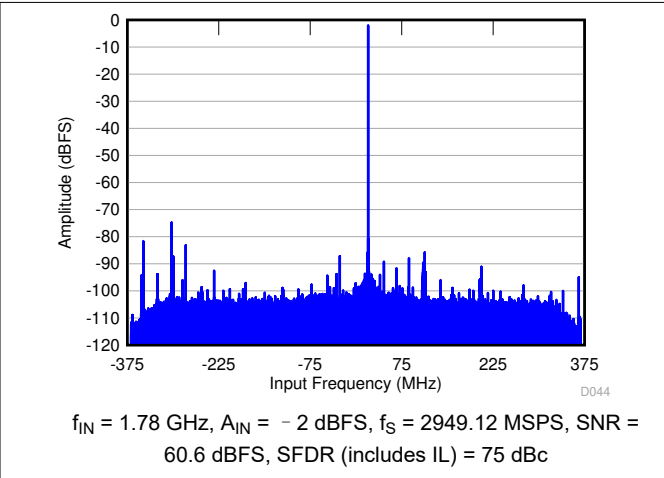
图 6-68. FFT in 4x Decimation (Complex Output)
