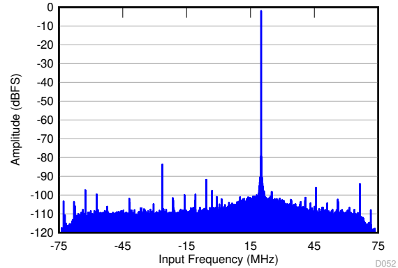
f_{IN} = 1.78 \text{ GHz} , A_{IN} = -2 \text{ dBFS} , f_S = 2949.12 \text{ MSPS} , SNR = 64.4 dBFS, SFDR (includes IL) = 84 dBc
