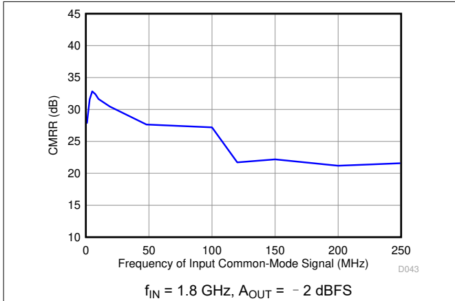
图 6-67. Common-Mode Rejection Ratio vs. Tone Frequency
