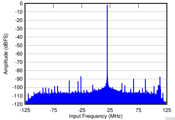
f_{IN} = 1.78 \text{ GHz} , A_{IN} = -2 \text{ dBFS} , f_S = 2949.12 \text{ MSPS} , SNR = 63.7 dBFS, SFDR (includes IL) = 83 dBc
