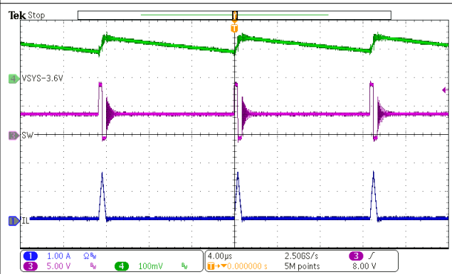
图 9-4. Power-Up with Charge Enabled
