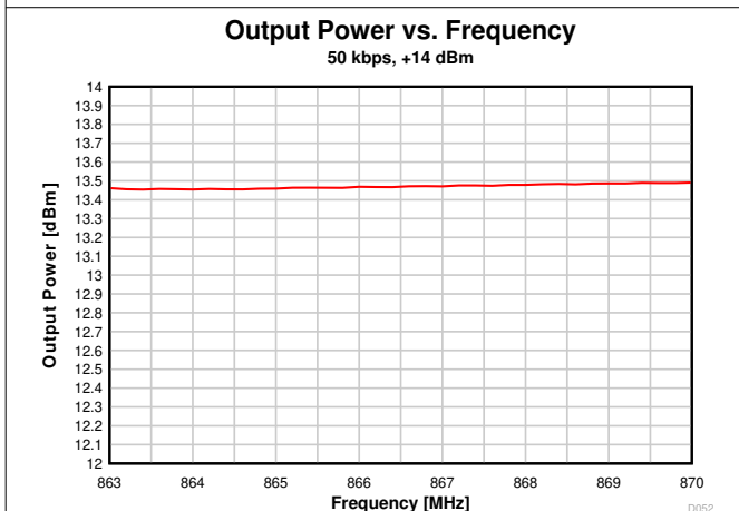
图 7-20. Output Power vs. Frequency (50 kbps, 868 MHz)
