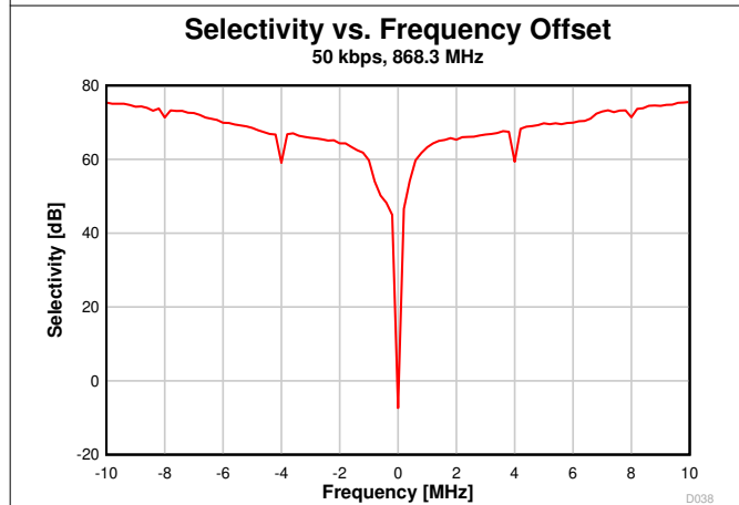
图 7-14. Selectivity vs. Frequency Offset (50 kbps, 868.3 MHz)
