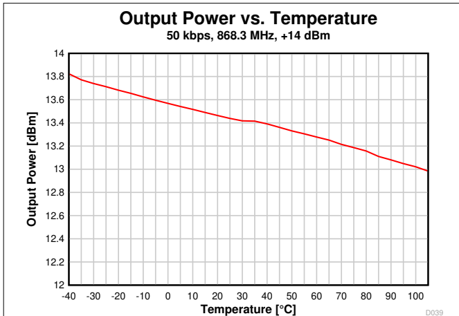
图 7-18. Output Power vs. Temperature (50 kbps, 868.3 MHz)
