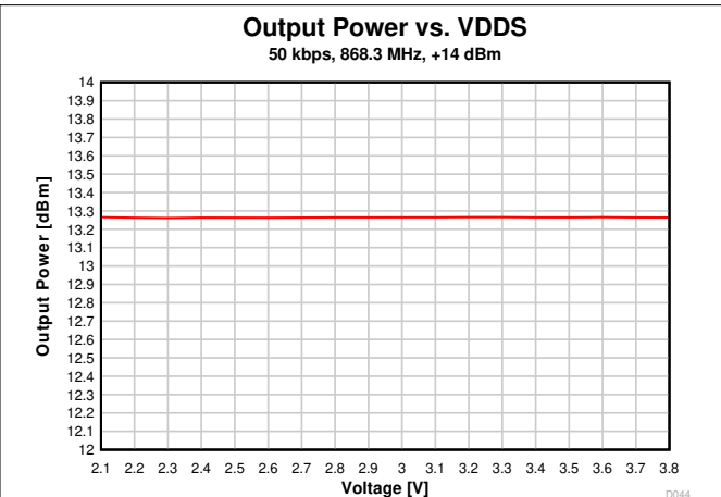
图 7-19. Output Power vs. Supply Voltage (VDD5) (50 kbps, 868.3 MHz)
