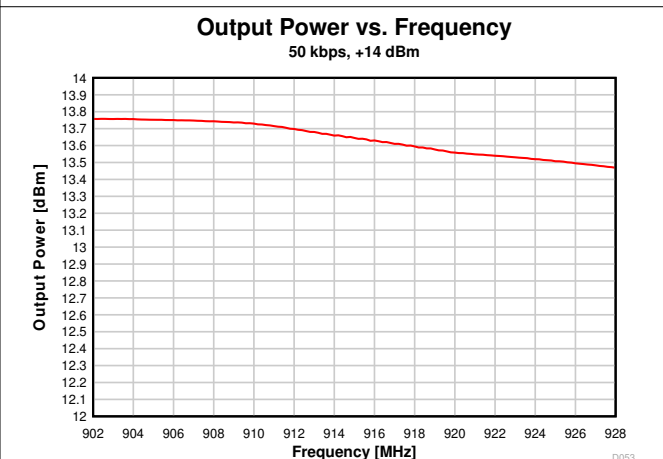
图 7-21. Output Power vs. Frequency (50 kbps, 915 MHz)
