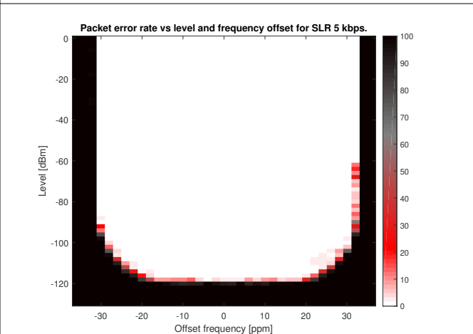
图 7-15. PER vs. Level vs. Frequency (SimpleLink™ Long Range 5 kbps, 868 MHz)
