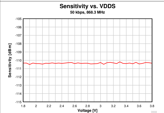
图 7-13. Sensitivity vs. Supply Voltage (VDD) (50 kbps, 868.3 MHz)
