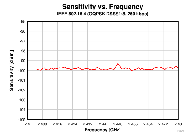
图 7-23. Sensitivity vs. Frequency (250 kbps, 2.44 GHz)
