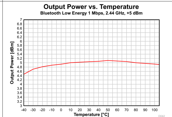
图 7-38. Output Power vs. Temperature (Bluetooth Low Energy 1 Mbps, 2.44 GHz, +5 dBm)
