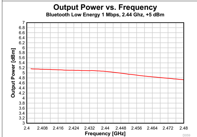
图 7-51. Output Power vs. Frequency (Bluetooth Low Energy 1 Mbps, 2.44 GHz, +5 dBm)
