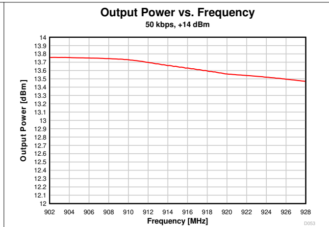
图 7-48. Output Power vs. Frequency (50 kbps, 915 MHz)
