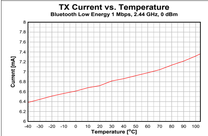
图 7-12. TX Current vs. Temperature (Bluetooth Low Energy 1 Mbps, 2.44 GHz)
