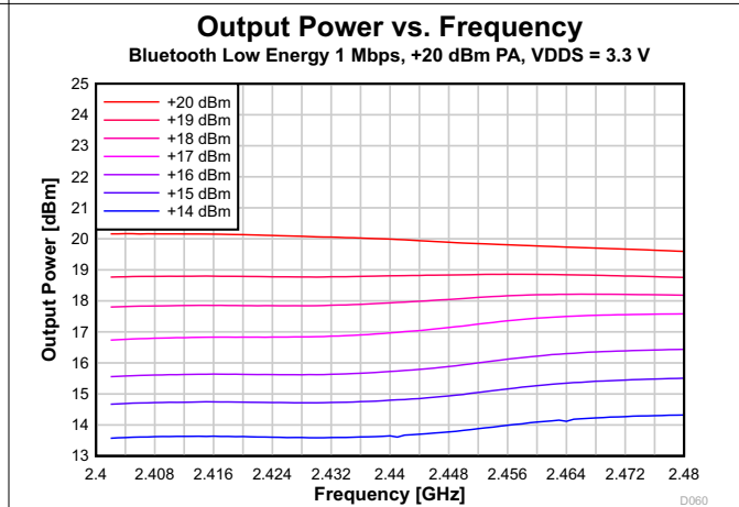
图 7-52. Output Power vs. Frequency (Bluetooth Low Energy 1 Mbps, 2.44 GHz, +20 dBm PA)
