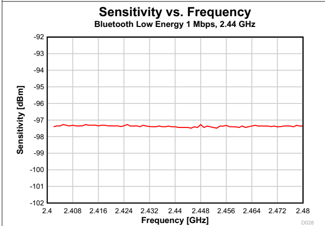
图 7-22. Sensitivity vs. Frequency (Bluetooth Low Energy 1 Mbps, 2.44 GHz)
