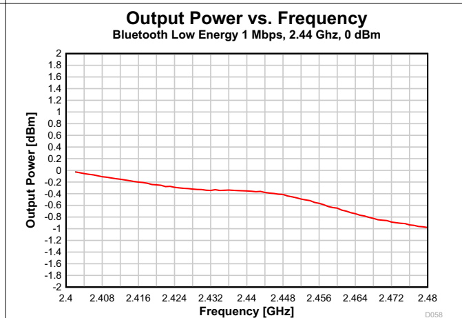
图 7-50. Output Power vs. Frequency (Bluetooth Low Energy 1 Mbps, 2.44 GHz)
