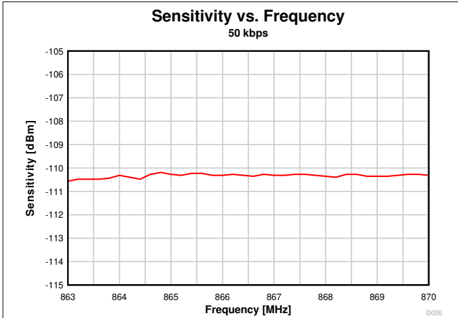
图 7-20. Sensitivity vs. Frequency (50 kbps, 868 MHz)
