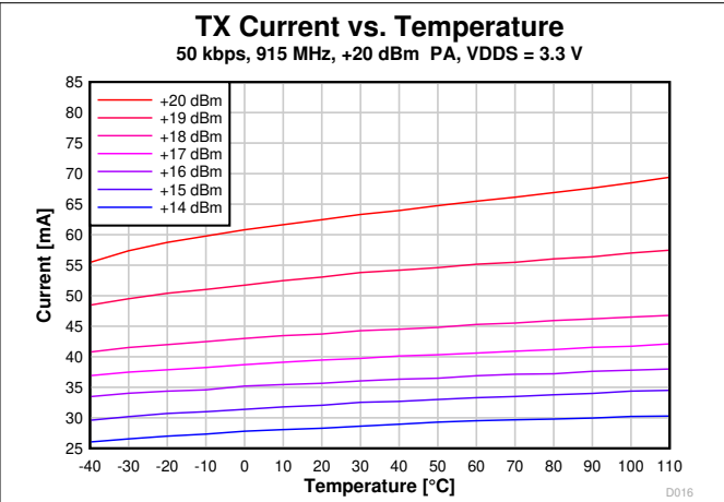
图 7-11. TX Current vs. Temperature (50 kbps, 915 MHz, VDD5 = 3.3 V)
