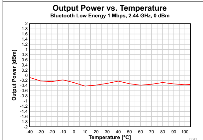
图 7-37. Output Power vs. Temperature (Bluetooth Low Energy 1 Mbps, 2.44 GHz)
