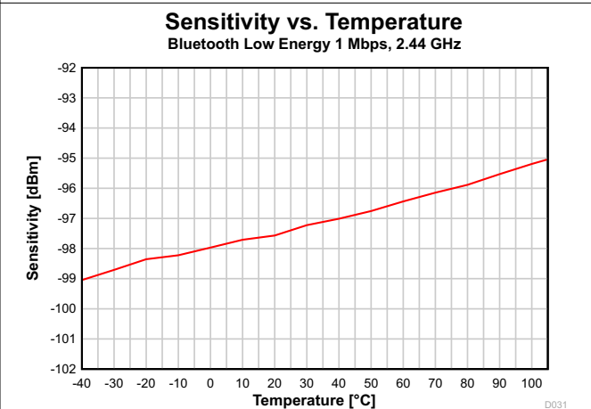
图 7-25. Sensitivity vs. Temperature (Bluetooth Low Energy 1 Mbps, 2.44 GHz)
