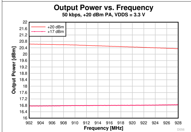
图 7-49. Output Power vs. Frequency (50 kbps, 915 MHz, VDD3 = 3.3 V)
