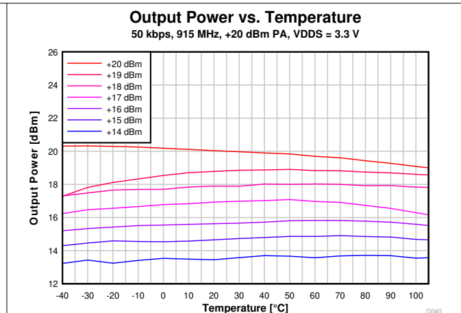
图 7-36. Output Power vs. Temperature (50 kbps, 915 MHz)
