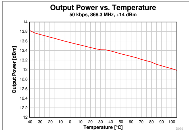
图 7-35. Output Power vs. Temperature (50 kbps, 868.3 MHz)
