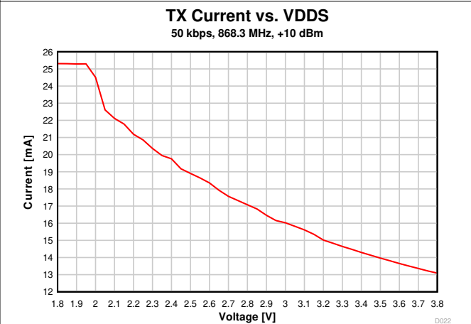
图 7-15. TX Current vs. Supply Voltage (VDD5) (50 kbps, 868.3 MHz)
