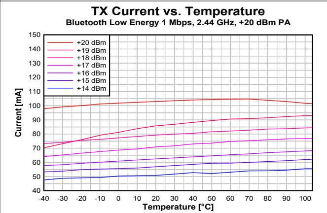
图 7-13. TX Current vs. Temperature (Bluetooth Low Energy 1 Mbps, 2.44 GHz, VDD5 = 3.3 V)
