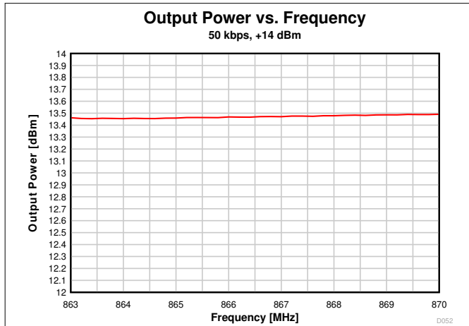
图 7-47. Output Power vs. Frequency (50 kbps, 868 MHz)
