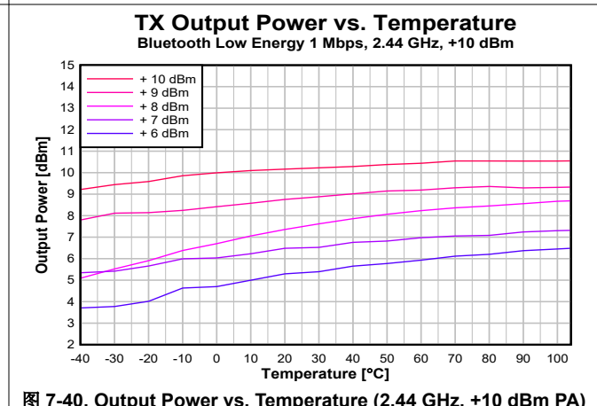
图 7-40. Output Power vs. Temperature (2.44 GHz, +10 dBm PA)
