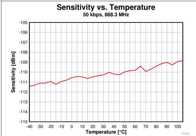
图 7-24. Sensitivity vs. Temperature (50 kbps, 868.3 MHz)
