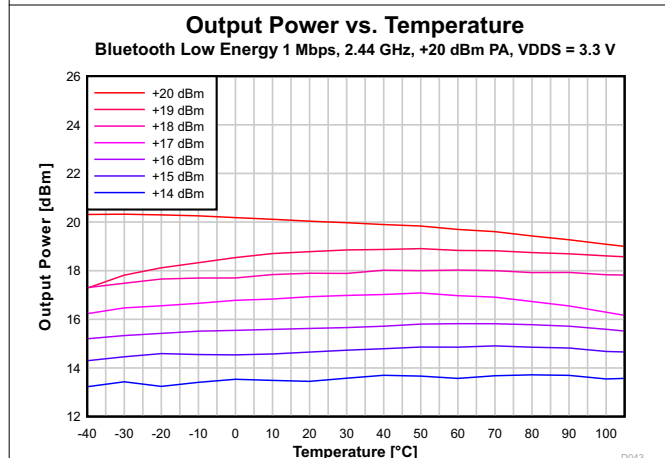
图 7-39. Output Power vs. Temperature (Bluetooth Low Energy 1 Mbps, 2.44 GHz, +20 dBm PA)
