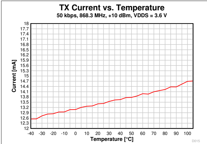
图 7-10. TX Current vs. Temperature (50 kbps, 868.3 MHz, VDD5 = 3.6 V)
