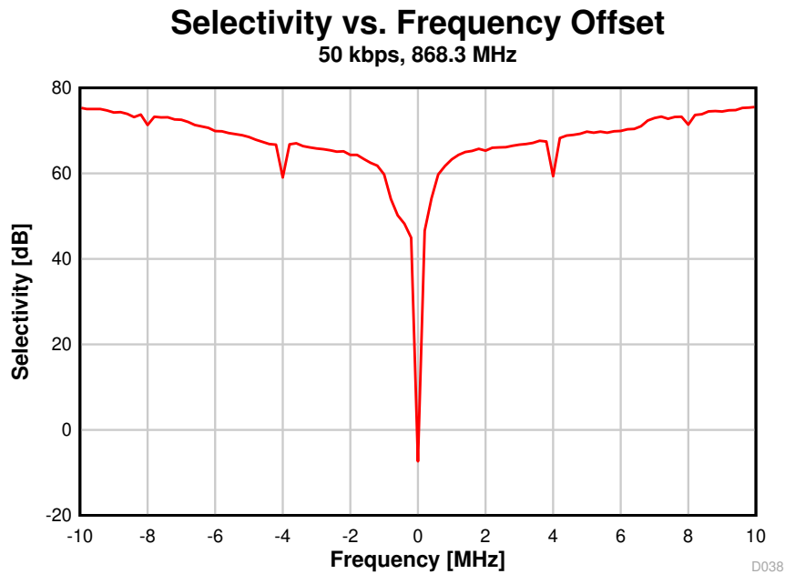
8-28. Selectivity vs. Frequency Offset (50 kbps, 868.3 MHz)
