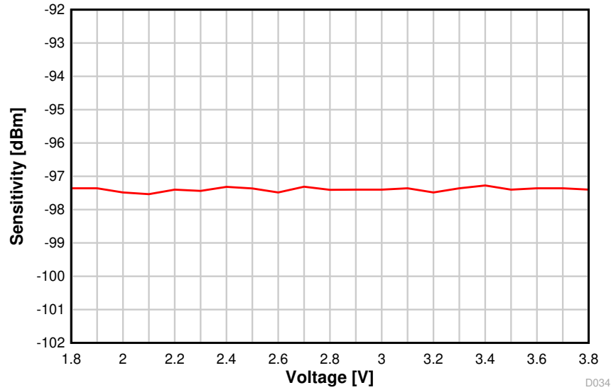
图 8-14. Sensitivity vs. Supply Voltage (VDDS) (BLE 1 Mbps, 2.44 GHz)
