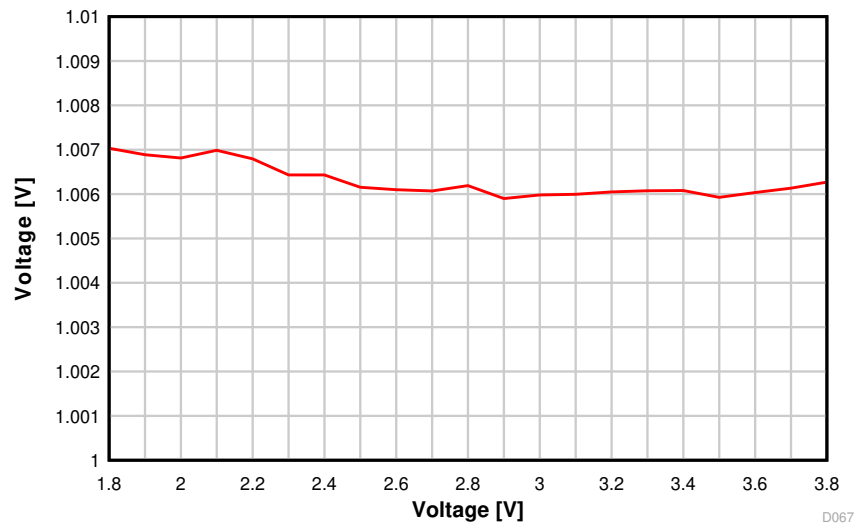
图 8-28. ADC Accuracy vs. Supply Voltage (VDD5)
