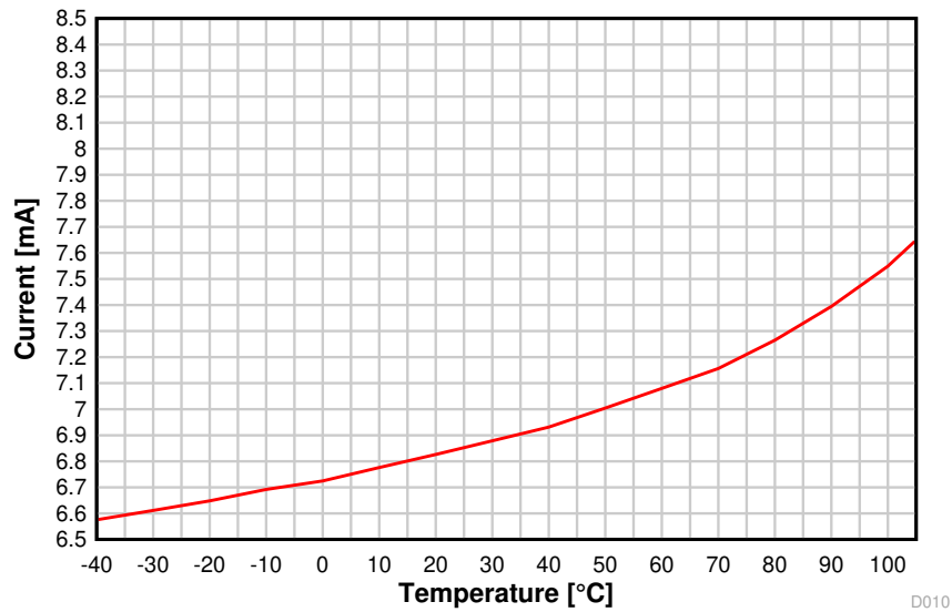
图 8-6. RX Current vs. Temperature (BLE 1 Mbps, 2.44 GHz)
