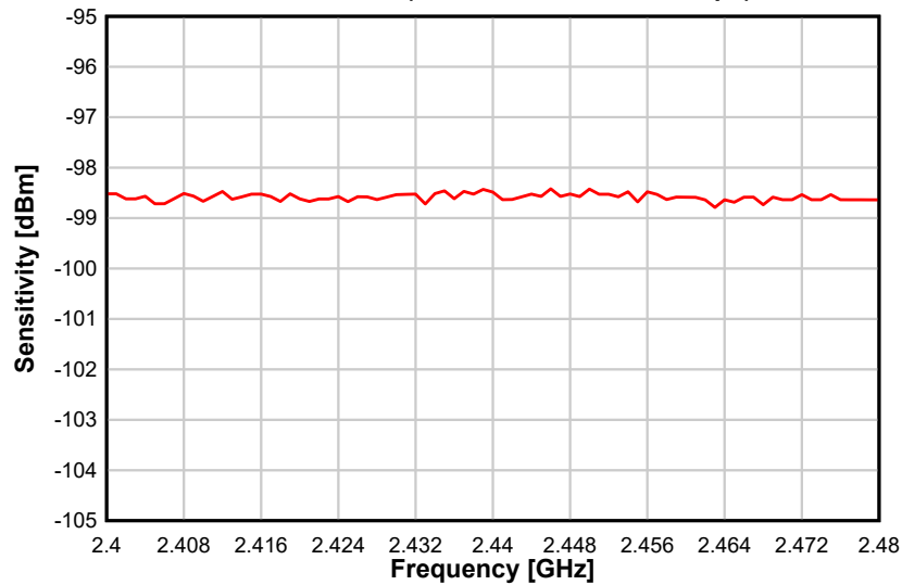
图 8-11. Sensitivity vs. Frequency (250 kbps, 2.44 GHz)
