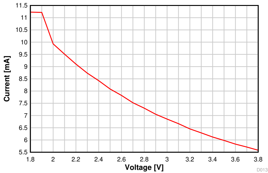
图 8-7. RX Current vs. Supply Voltage (VDD5) (BLE 1 Mbps, 2.44 GHz)
