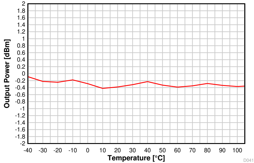
图 8-17. Output Power vs. Temperature (BLE 1 Mbps, 2.44 GHz)
