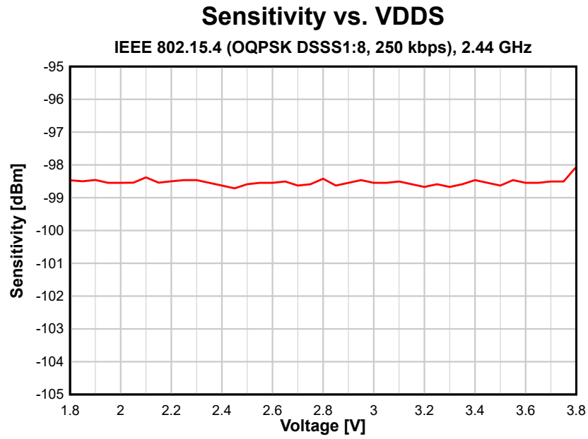
图 8-16. Sensitivity vs. Supply Voltage (VDDS) (250 kbps, 2.44 GHz)
