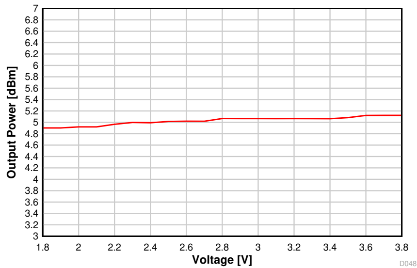
图 8-20. Output Power vs. Supply Voltage (VDDS) (BLE 1 Mbps, 2.44 GHz, +5 dBm)
