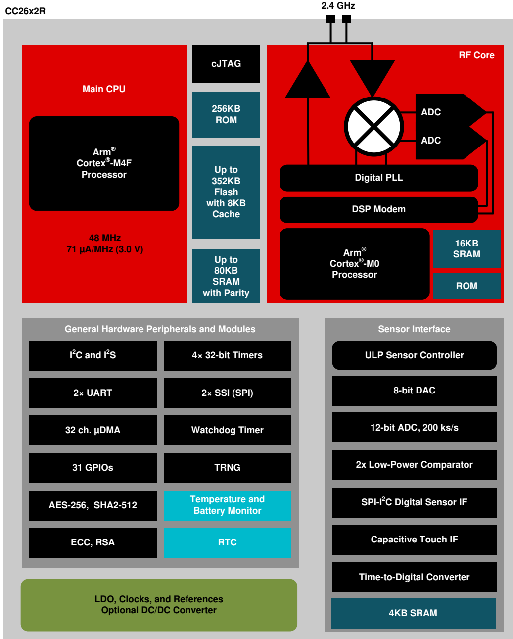
图 4-1. CC2652R Block Diagram
