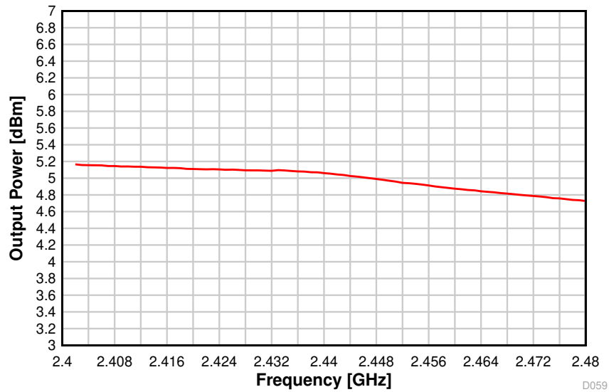
图 8-22. Output Power vs. Frequency (BLE 1 Mbps, 2.44 GHz, +5 dBm)
