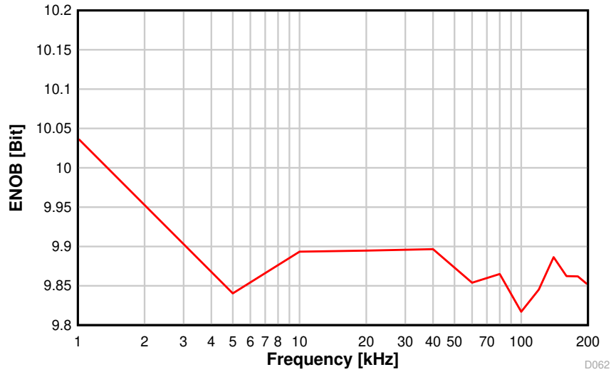
图 8-24. ENOB vs. Sampling Frequency
