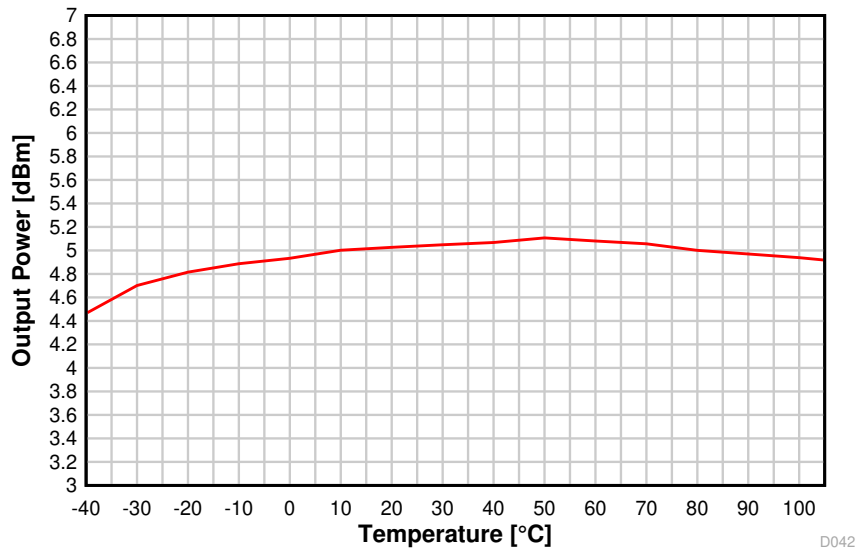
图 8-18. Output Power vs. Temperature (BLE 1 Mbps, 2.44 GHz, +5 dBm)
