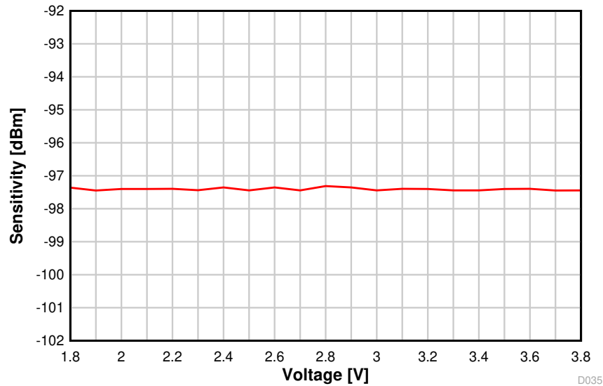
图 8-15. Sensitivity vs. Supply Voltage (VDDS) (BLE 1 Mbps, 2.44 GHz, DCDC Off)
