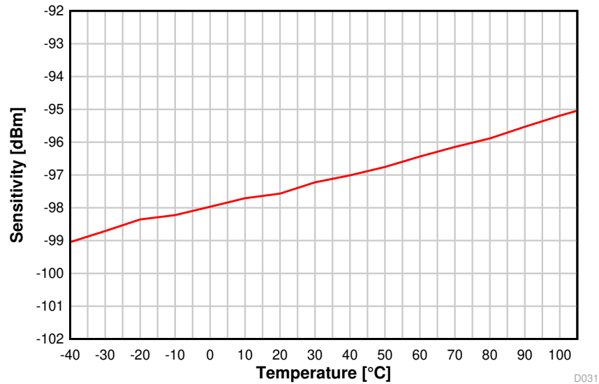
图 8-12. Sensitivity vs. Temperature (BLE 1 Mbps, 2.44 GHz)
