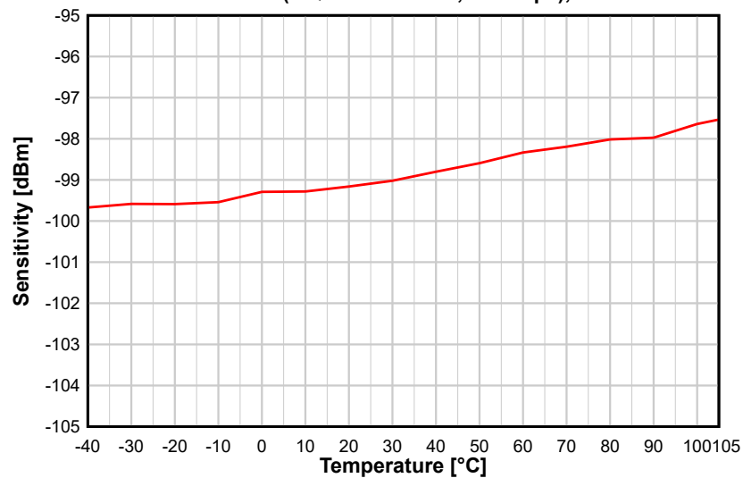
图 8-13. Sensitivity vs. Temperature (250 kbps, 2.44 GHz)
