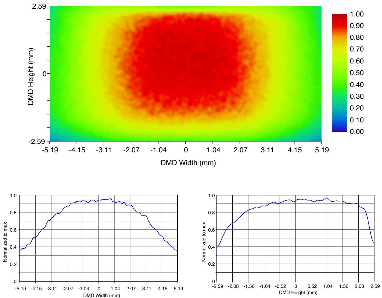
图 7-5. Non-Uniform Illumination Profile
