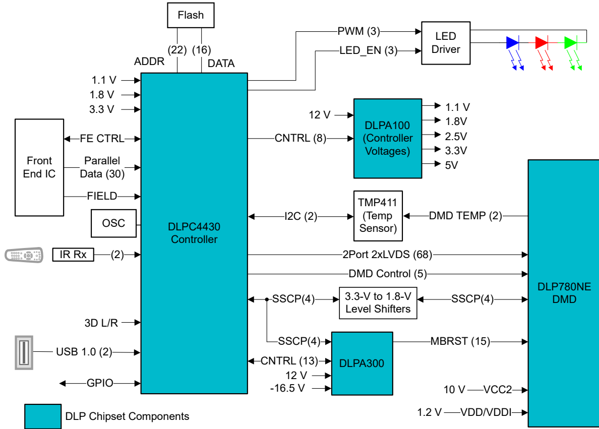
图 8-1. Typical Full HD LED Application
