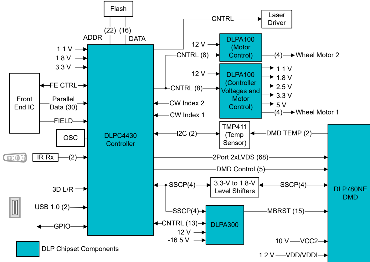
图 8-2. Typical Full HD Laser Phosphor Application
