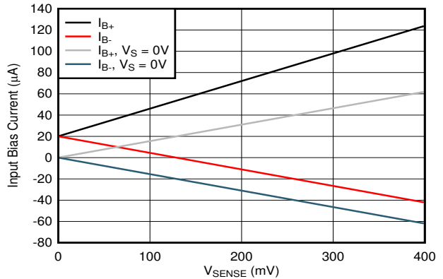
图 6-16. INA310x2, INA310x3 Input Bias Current vs V_{SENSE}
