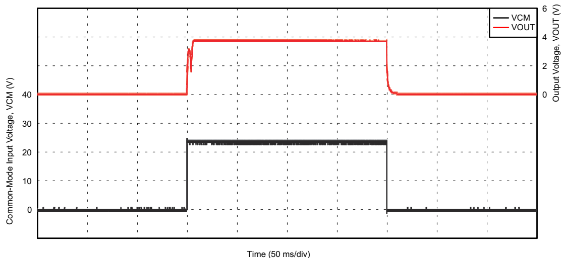
图 8-2. Solenoid Control Current Response
