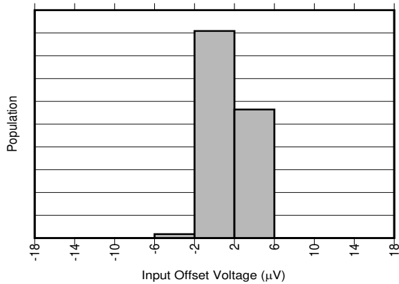
图 6-5. INA310A5 Input Offset Production Distribution
