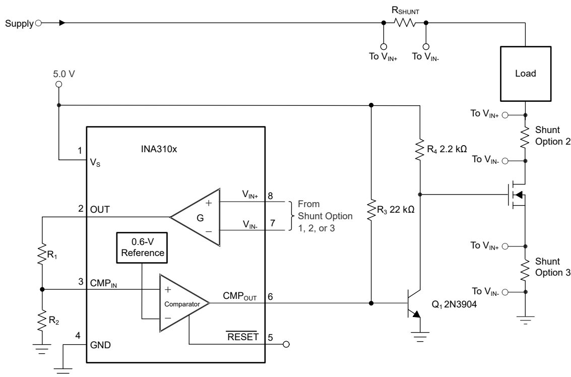
图 8-3. Low-Side Switch Overcurrent Shutdown
