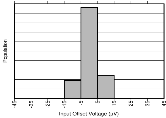
图 6-3. INA310A3 Input Offset Production Distribution
