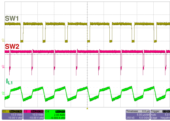
图 6-13. Forced CCM Operation (Buck-Boost)
