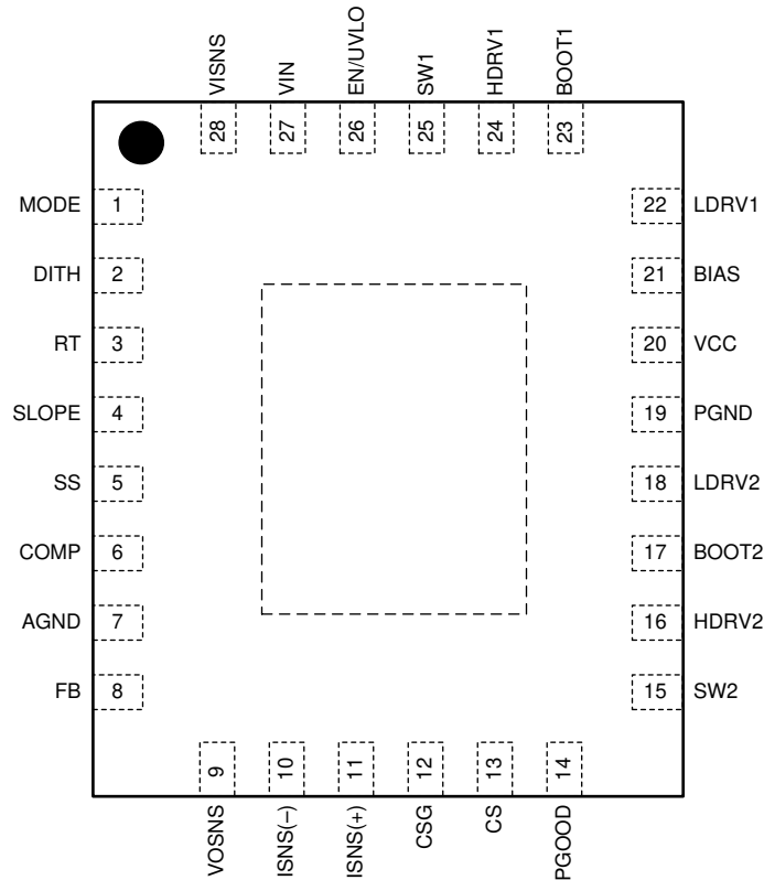
图 5-1. QFN-28 RHF Package Top View
