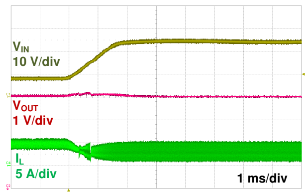
图 8-5. Line Transient Response (8 V - 24 V, I_{OUT} = 2 \text{ A} )
