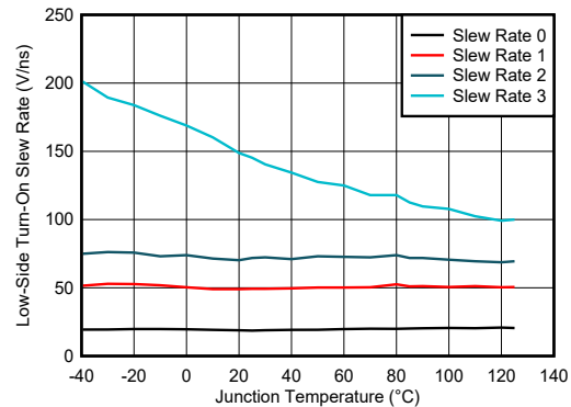
图 6-10. Low-Side Turn-On Slew Rate vs Junction Temperature
