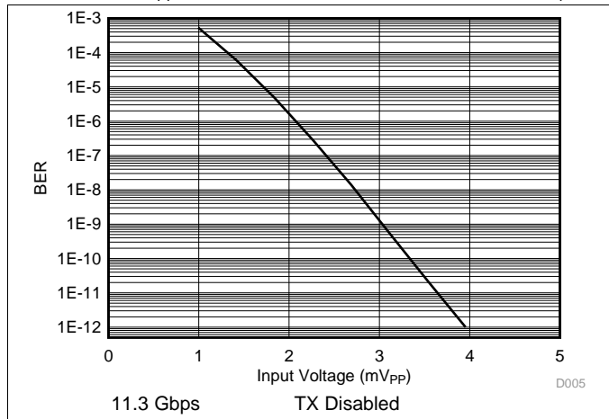
Figure 27. RX Bit-Error Ratio vs Input Amplitude
