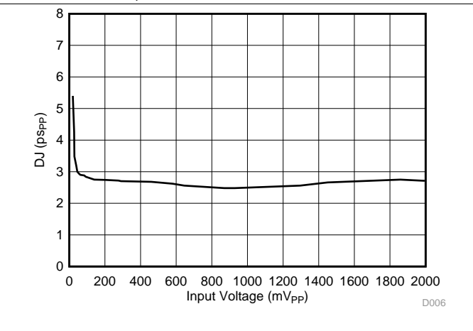
Figure 28. RX Deterministic Jitter vs Input Amplitude
