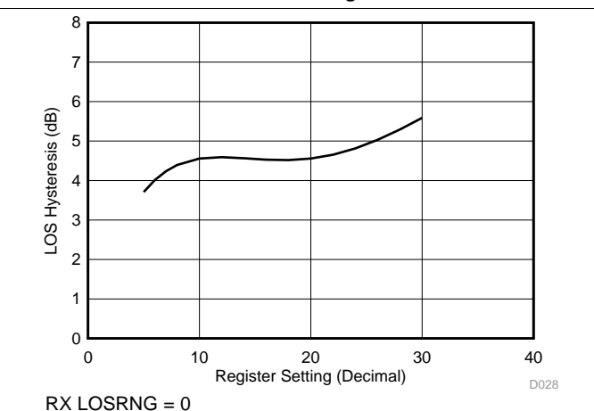
Figure 32. LOS Hysteresis vs Register 7 Setting
