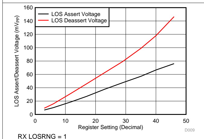
Figure 31. LOS Assert / Deassert Voltage vs Register 7 Setting
