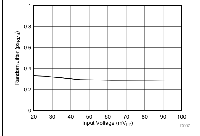
Figure 29. RX Random Jitter vs Input Amplitude
