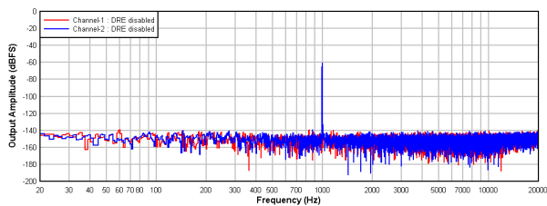
图 9-4. PCM1820-Q1: FFT With a -60-dBr Input With DRE Disabled
