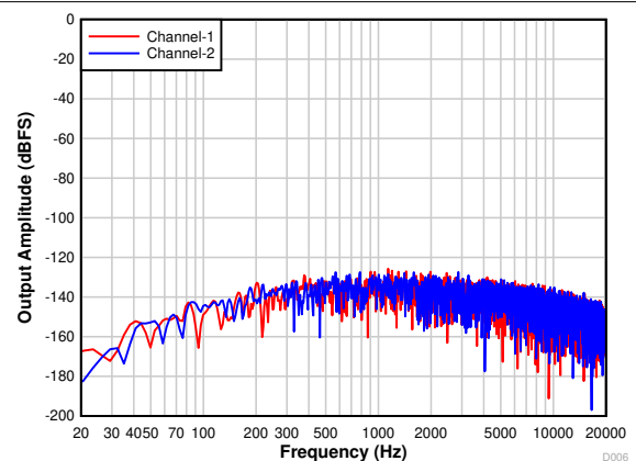
图 7-18. PCM1821-Q1: FFT With Idle Input and DRE Disabled
