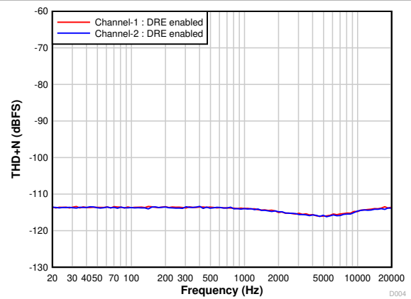
图 7-4. PCM1820-Q1: THD+N vs Input Frequency With a -60-dBr Input
