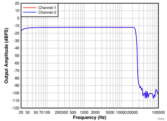
图 7-6. PCM1820: Frequency Response With a -12-dBr Input
