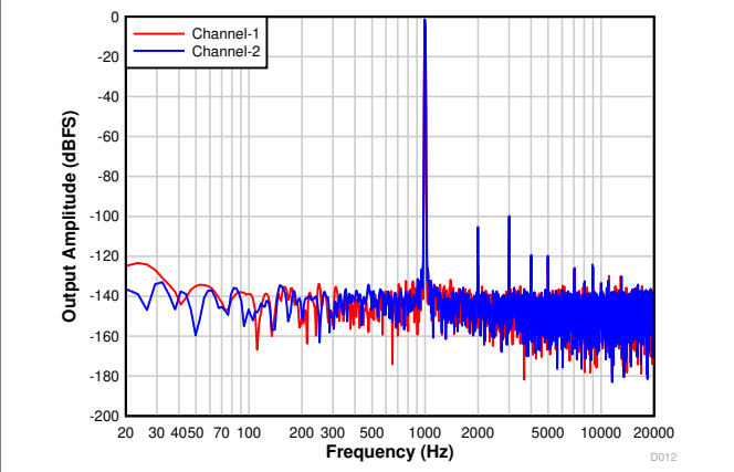
图 7-12. PCM1820: FFT With a -1-dBr Input
