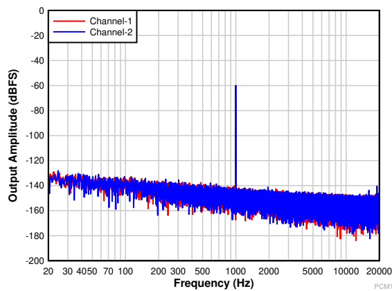
9-6. PCM1821: FFT With a -60-dBr Input
