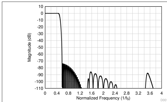
图 8-17. Linear Phase Decimation Filter Magnitude Response
