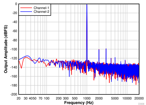
图 7-20. PCM1821: FFT With a -1-dBr Input
