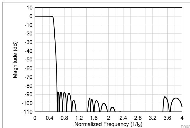
图 8-21. Low-Latency Decimation Filter Magnitude Response
