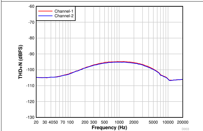
图 7-15. PCM1821: THD+N vs Input Frequency With a -1-dBr Input
