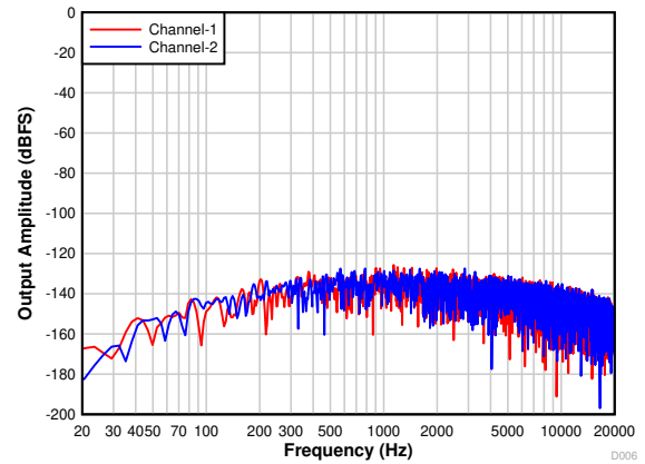
图 7-18. PCM1821: FFT With Idle Input
