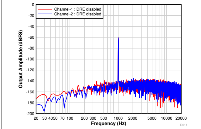
图 7-11. PCM1820: FFT With a -60-dBr Input and DRE Disabled
