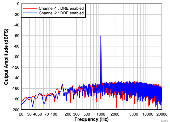
图 7-10. PCM1820: FFT With a -60-dBr Input and DRE Enabled
