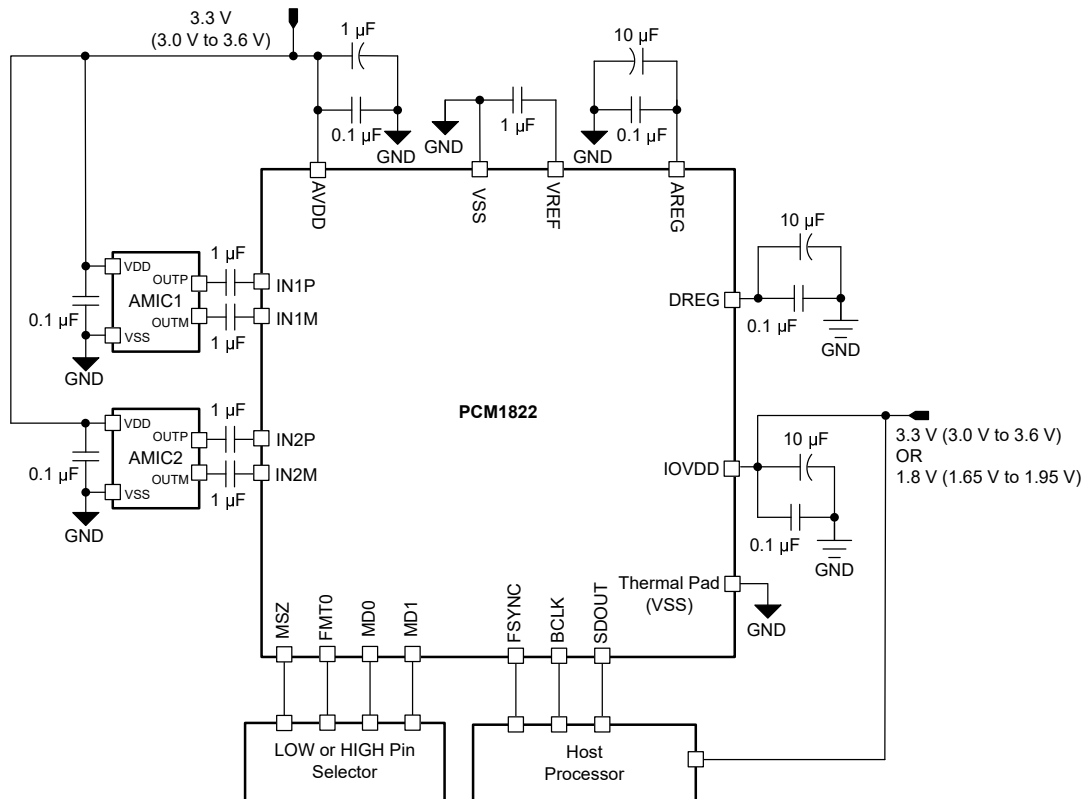
图 9-1. Two-Channel Analog Microphone Recording Diagram for 3.3-V AVDD Operation
