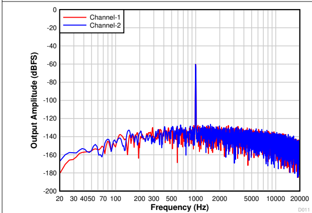
图 7-14. Differential FFT With a -60-dBr Input
