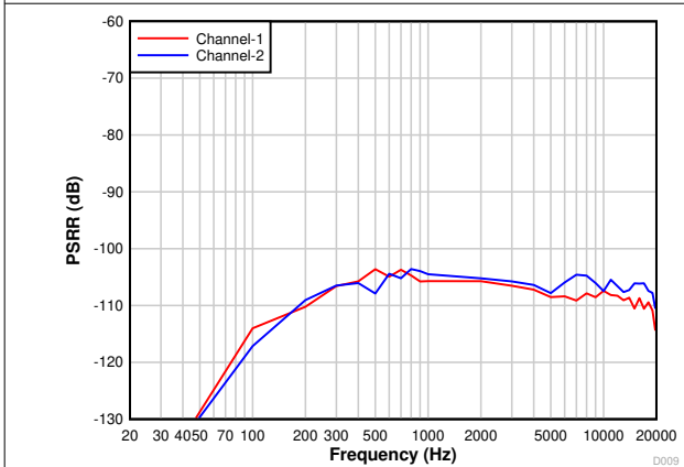
图 7-12. Power-Supply Rejection Ratio vs Ripple Frequency With 100-mVPP Amplitude
