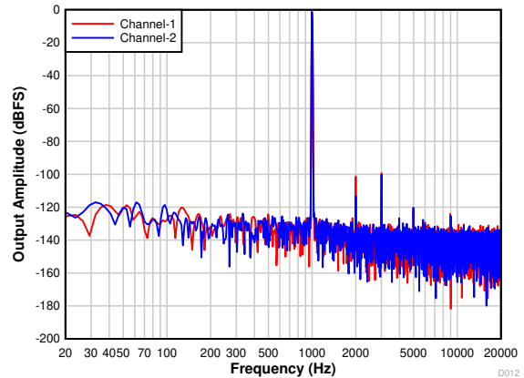
图 7-17. Differential FFT With a - 1-dBr Input
