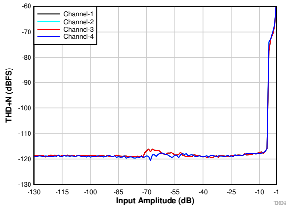
图 7-18. PDM Input THD+N vs Input Amplitude
