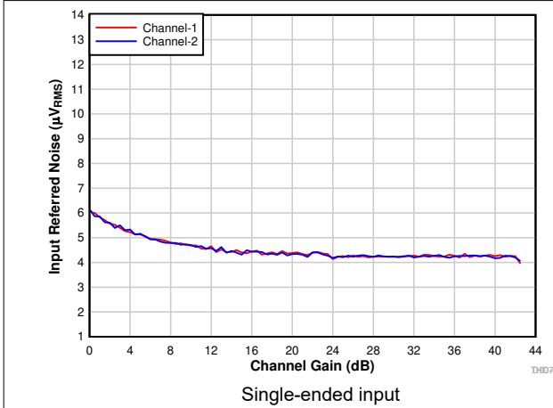
图 7-10. Input-Referred Noise vs Channel Gain
