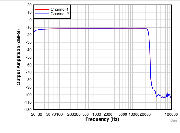
图 7-11. Frequency Response With a -12-dBr Input
