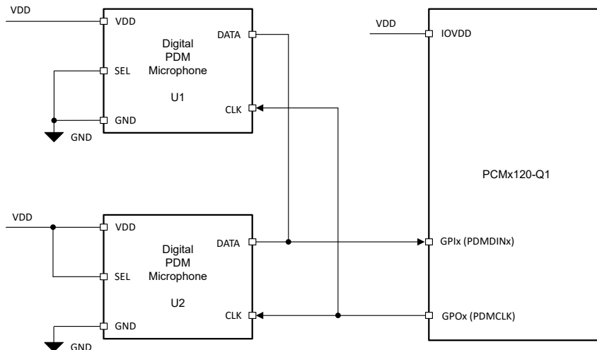
图 8-64. Digital PDM Microphones Connection Diagram for the PCM3120-Q1
