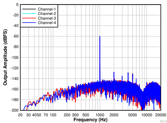
图 7-20. PDM Input FFT With a - 60-dBr Input
