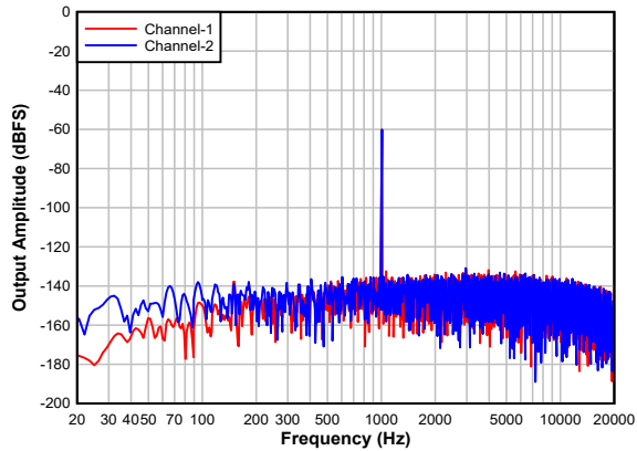
图 7-16. Single Ended FFT With a - 60-dBr Input
