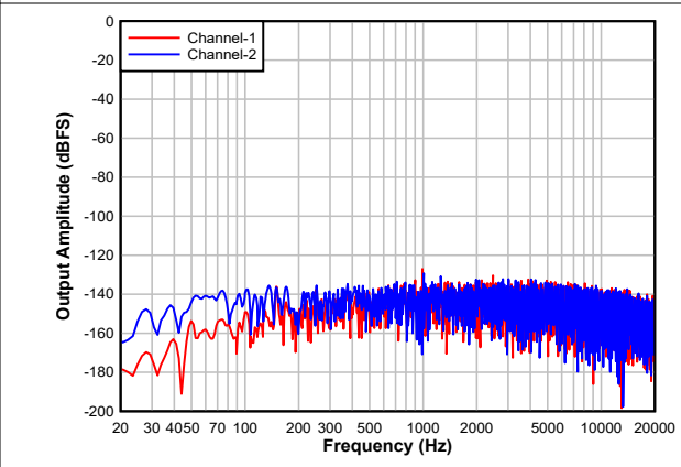
图 7-15. Single Ended FFT With Idle Input
