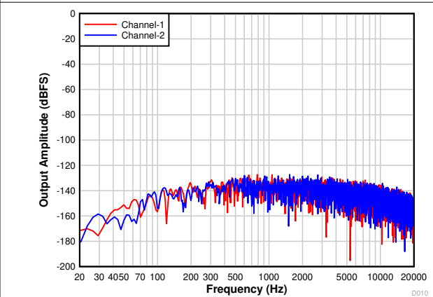
图 7-13. Differential FFT With Idle Input
