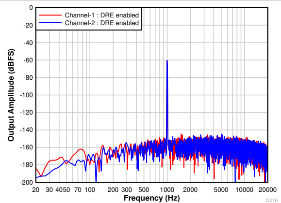
图 7-19. Differential FFT With a -60-dBr Input With DRE Enabled
