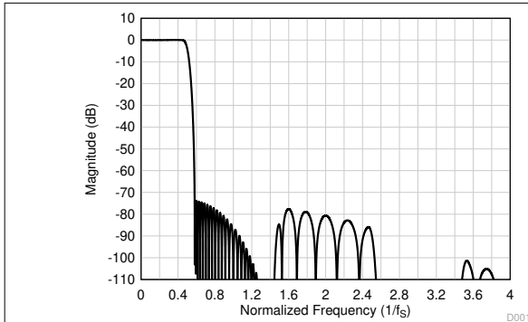
图 8-25. Linear Phase Decimation Filter Magnitude Response
