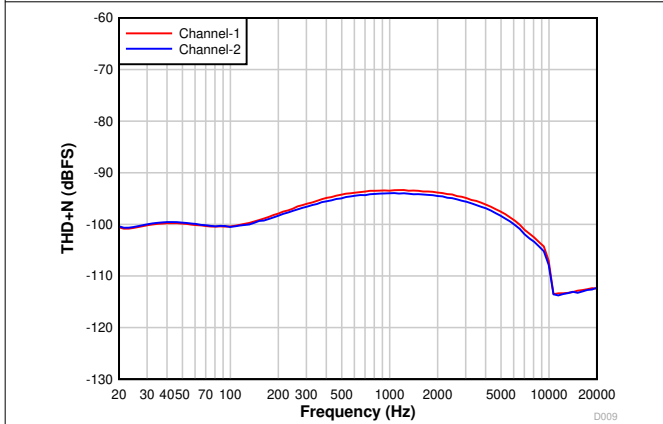
图 7-10. THD+N vs Input Frequency at -60-dBr Input With DRE Enabled
