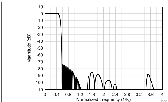
图 8-27. Linear Phase Decimation Filter Magnitude Response
