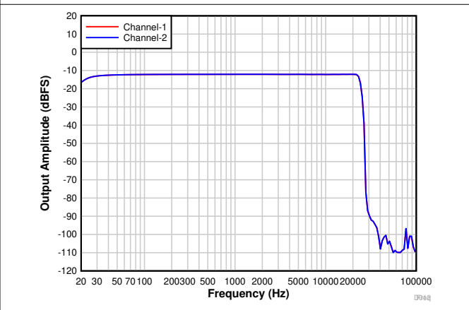
图 7-15. Frequency Response With a -12-dBr Input
