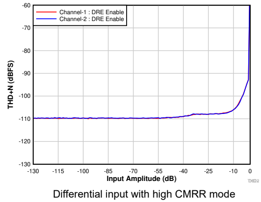
图 7-29. THD+N vs Input Amplitude With DRE Enabled
