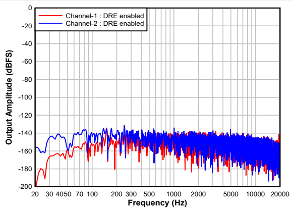
图 7-21. Single Ended FFT With Idle Input With DRE Enabled
