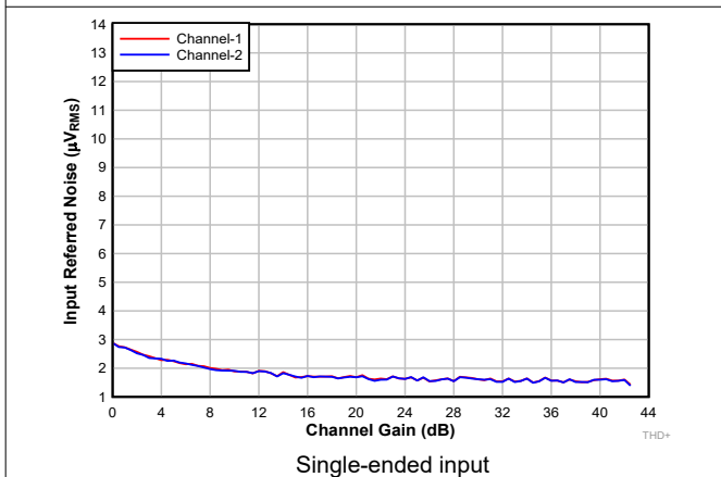
图 7-14. Input-Referred Noise vs Channel Gain
