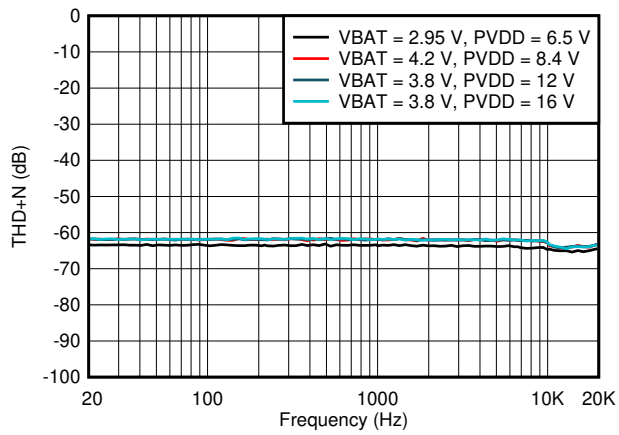
图 6-39. V Sense THDN vs Frequency
