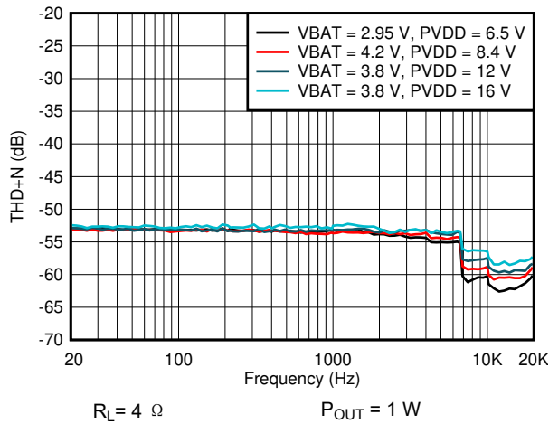
图 6-33. I Sense THDN vs Frequency
