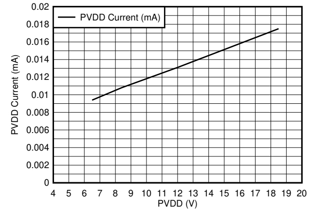
图 6-28. PVDD Idle Current vs PVDD
