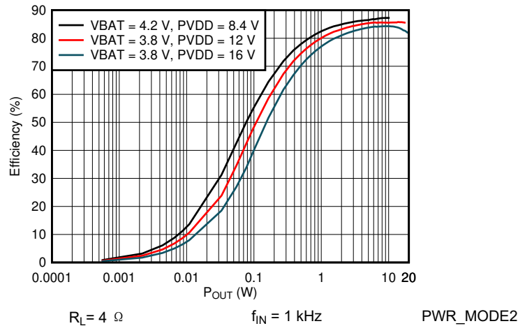
图 6-21. Efficiency vs Output Power
