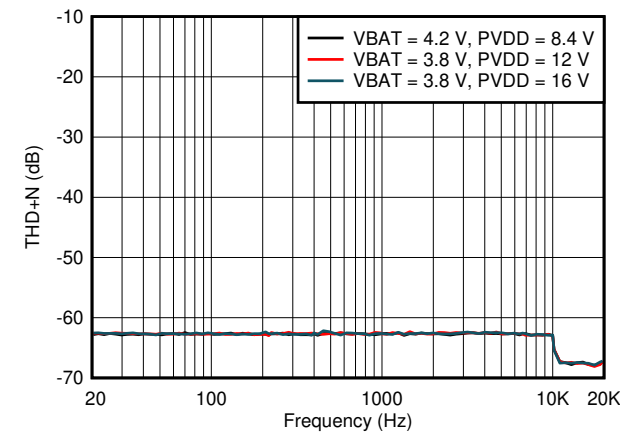
图 6-40. V Sense THDN vs Frequency
