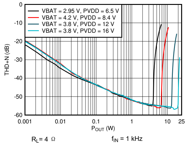
图 6-29. I Sense THDN vs Output Power
