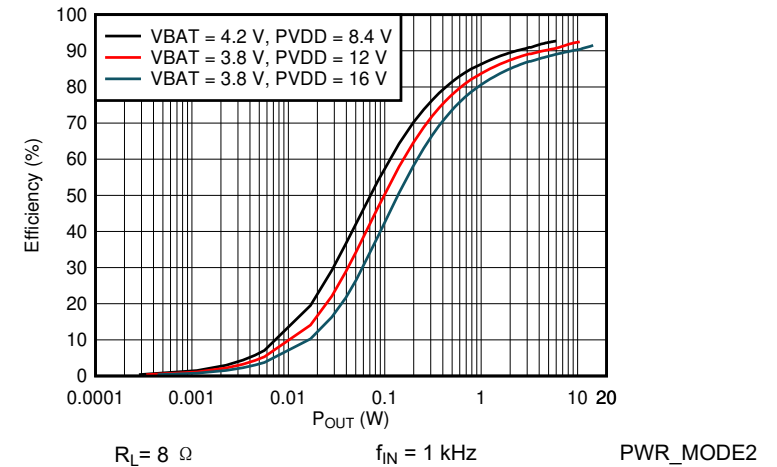
图 6-22. Efficiency vs Output Power
