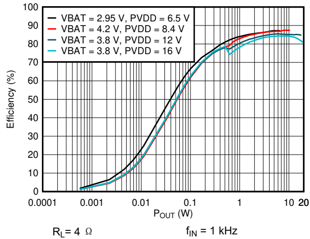
图 6-19. Efficiency vs Output Power
