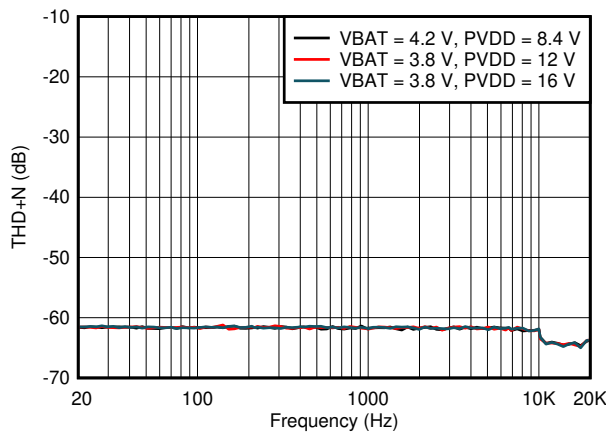
图 6-39. V Sense THDN vs Frequency
