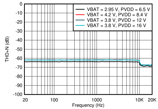
图 6-40. V Sense THDN vs Frequency
