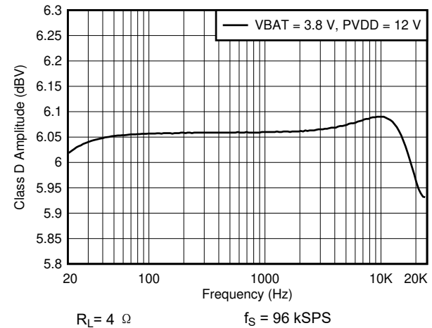
图 6-18. Class D Frequency Response
