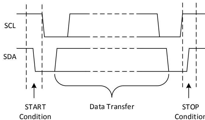
图 8-1. Definition of Start and Stop Conditions
