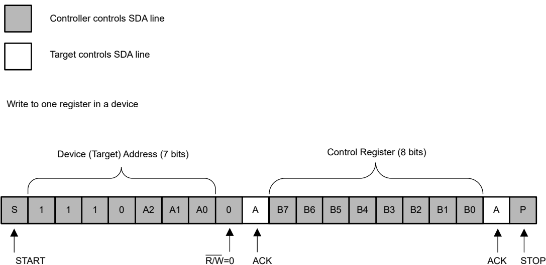
图 8-4. Write to Register
