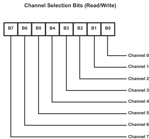
Figure 8-6. Control Register
