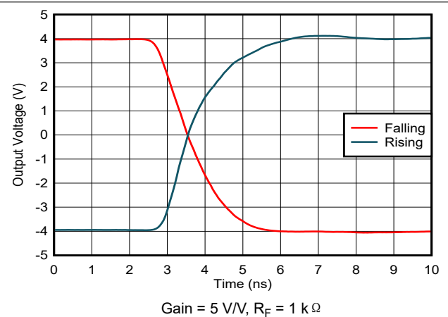
图 7-18. Settling Time
