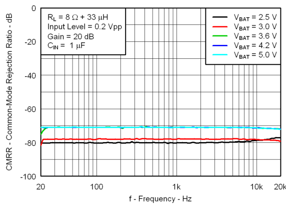
图 21. Common Mode Rejection Ratio vs Frequency
