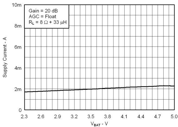
图 19. Quiescent Supply Current vs Supply Voltage
