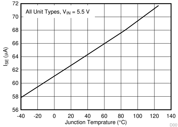
图 6-13. Enabled Supply Current ( I_{SE} ) vs Temperature
