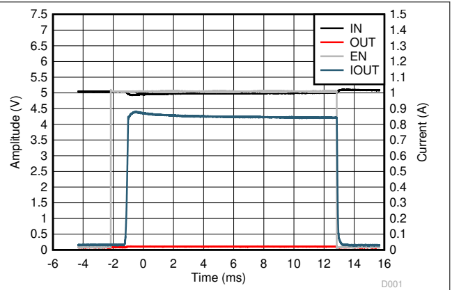
图 6-2. Enable into Short
