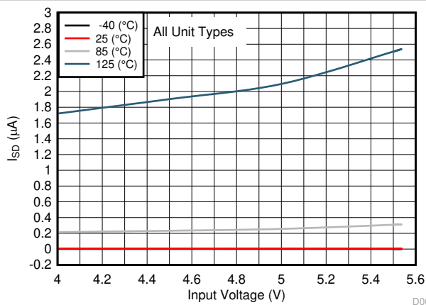
图 6-11. Disabled Supply Current ( I_{SD} ) vs Input Voltage
