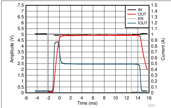
图 6-1. Turn ON into 10 Ω
