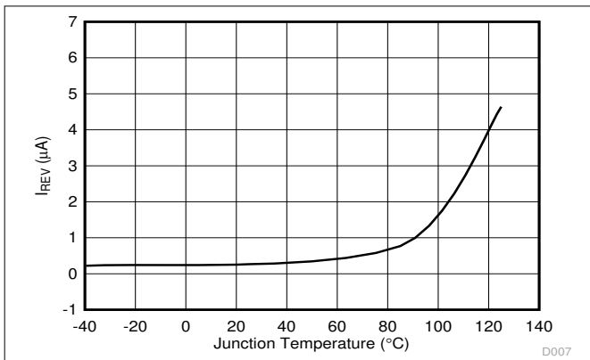
图 6-5. Reverse Leakage Current ( I_{REV} ) vs Temperature
