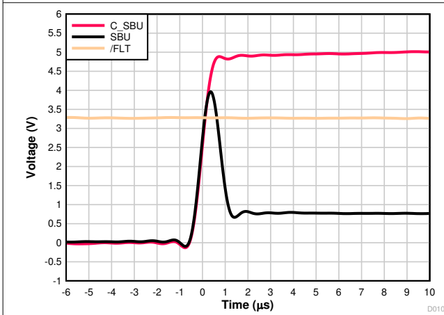
图 7-5. SBU Short-to- V_{BUS} 5 V Zoomed In
