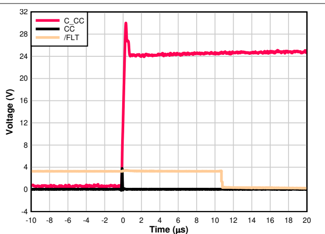
图 7-18. CC Short-to-V BUS 24 V Zoomed Out
