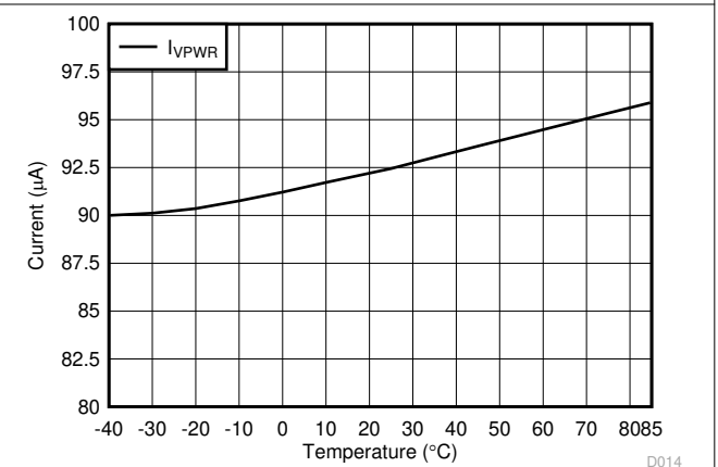
图 7-30. V PWR Supply Leakage vs Ambient Temperature at 3.6 V
