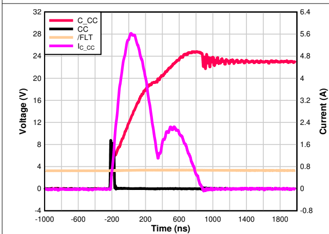
图 7-17. CC Short-to-V BUS 24 V Zoomed In
