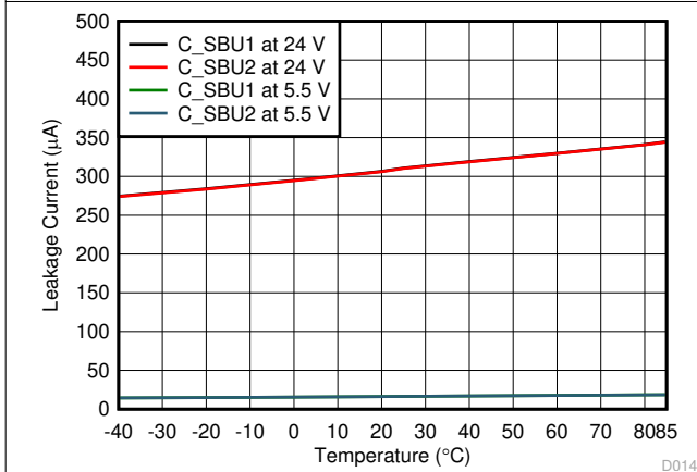
图 7-11. C_SBU OVP Leakage Current vs Ambient Temperature at 5.5 V and 24 V
