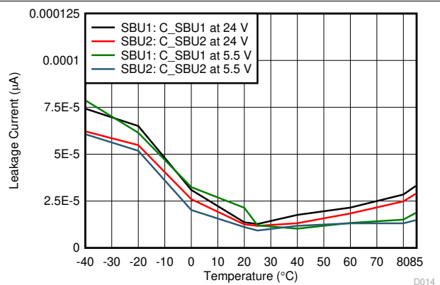
图 7-12. SBU OVP Leakage Current vs Ambient Temperature at 5.5 V and 24 V
