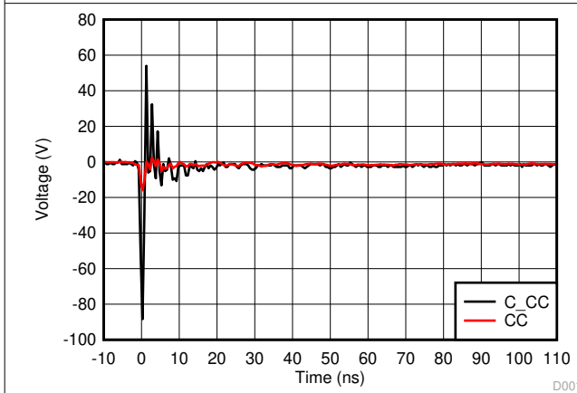
图 7-23. CC IEC 61000-4-2 -8-kV Response Waveform
