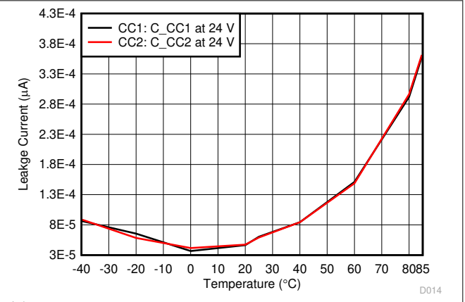
图 7-26. CC OVP Leakage Current vs Ambient Temperature at C CC = 24 V
