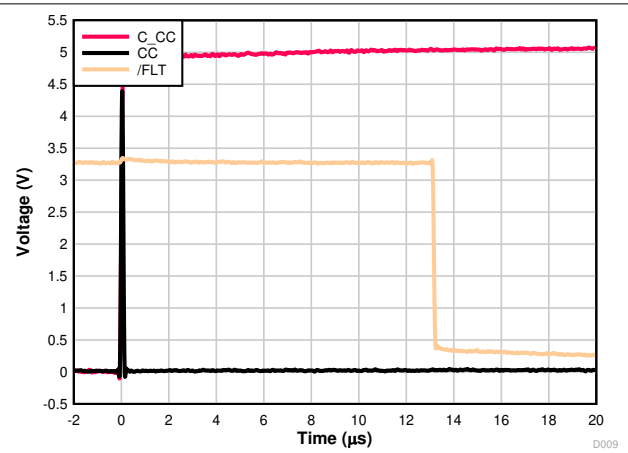
图 7-20. CC Short-to- V_{BUS} 5 V Zoomed Out
