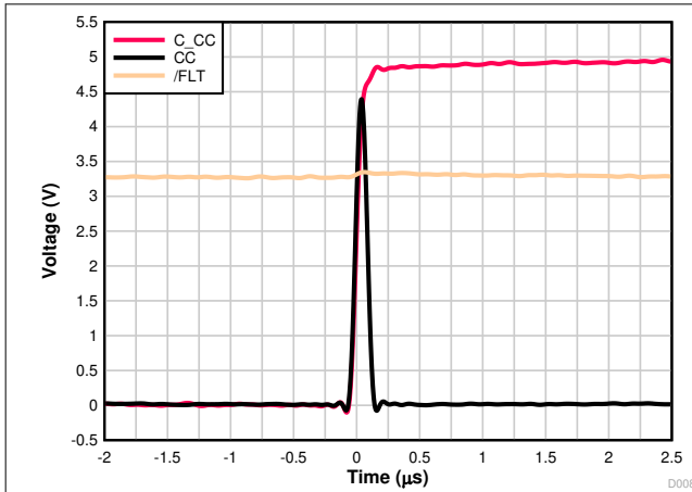
图 7-19. CC Short-to- V_{BUS} 5 V Zoomed In
