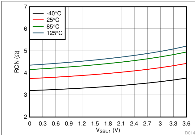
图 7-7. SBU R ON Flatness
