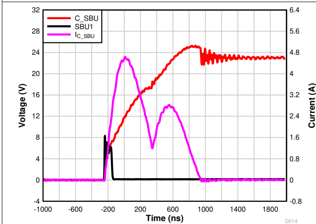
图 7-3. SBU Short-to- V_{BUS} 24 V Zoomed In
