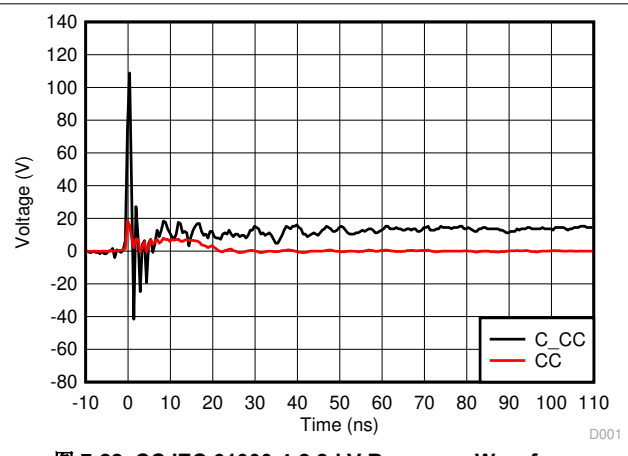
图 7-22. CC IEC 61000-4-2 8-kV Response Waveform
