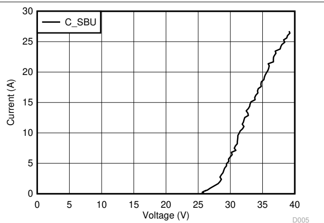
图 7-14. C_SBU TLP Curve Unpowered
