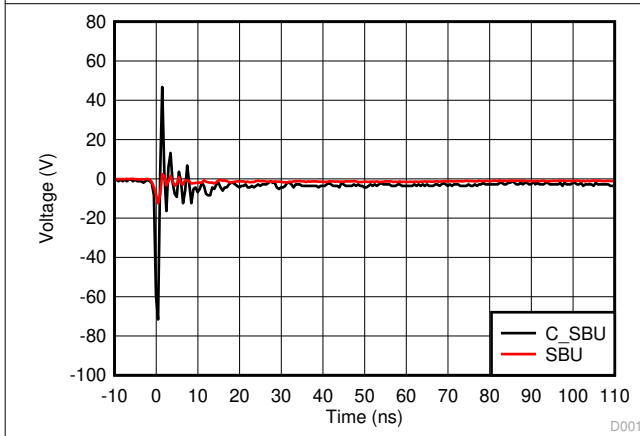
图 7-9. SBU IEC 61000-4-2 -4-kV Response Waveform
