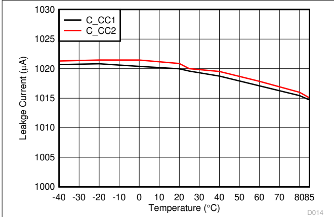
图 7-25. C CC OVP Leakage Current vs Ambient Temperature at C CC = 24 V
