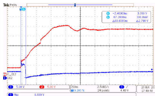
图 9-4. TPD4S311 Protecting the TPS65982 During a Short-to- V_{BUS} Event
