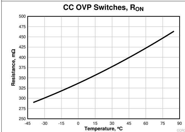
图 7-21. CC R_{ON} Versus Temperature
