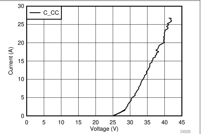
图 7-28. C CC TLP Curve Unpowered
