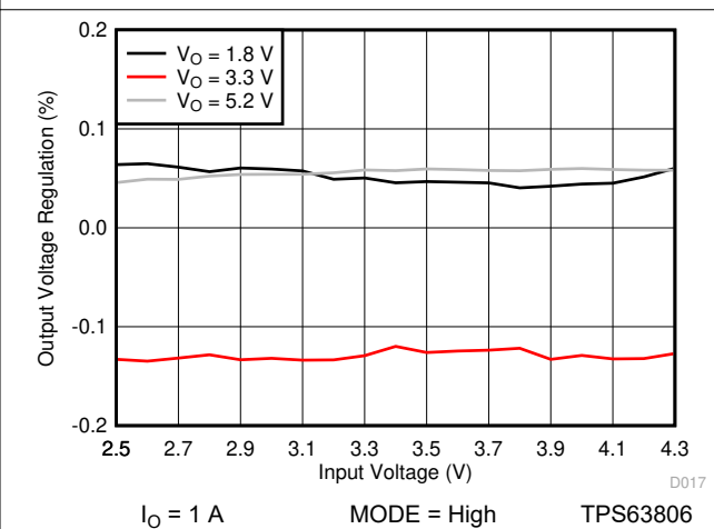
图 10-26. Line Regulation (PFM/PWM)
