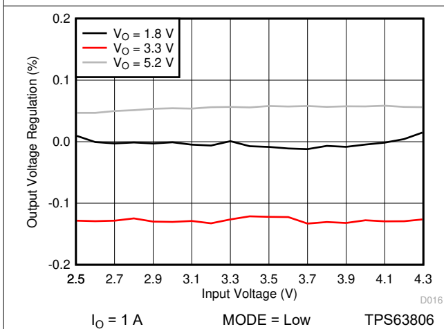
图 10-25. Line Regulation (PWM Only)
