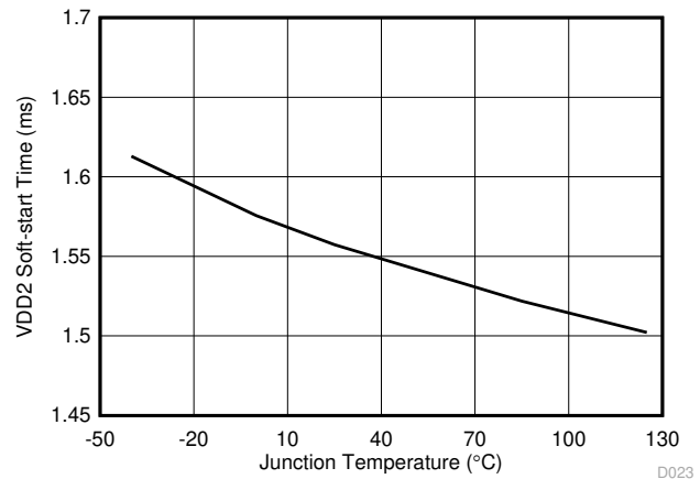
图 6-22. VDD2 Soft-Start Time vs Junction Temperature
