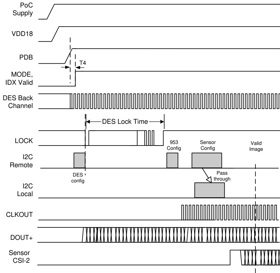
图 9-2. Initialization Sequence: Synchronous Cloning Mode
