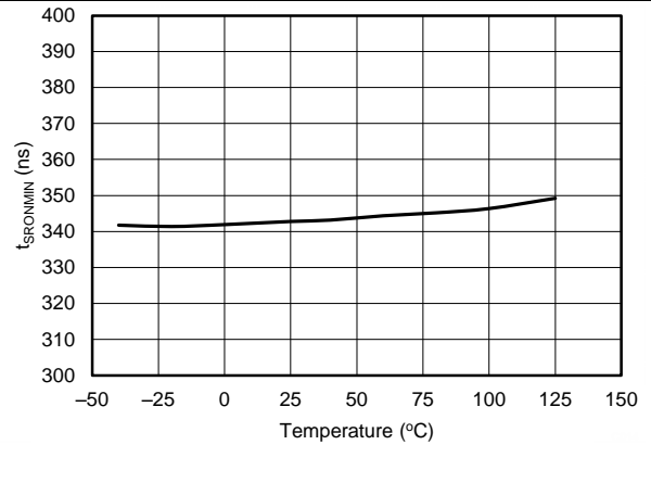
Figure 10. DRV Minimum On Time vs Temperature
