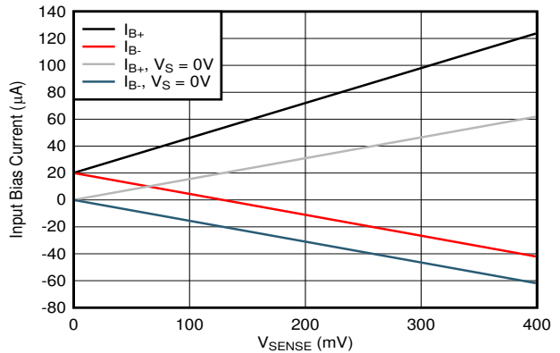
Figure 6-16. INA310x2, INA310x3 Input Bias Current vs V_{SENSE}
