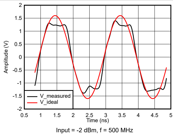
Figure 6-35. Overdrive Recovery
