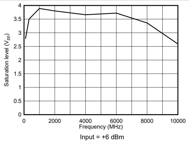
Figure 6-36. Saturation Voltage
