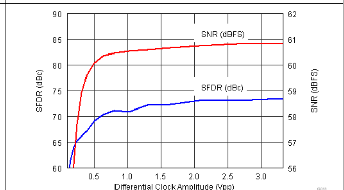
图 7-23. Performance Across Clock Amplitude
