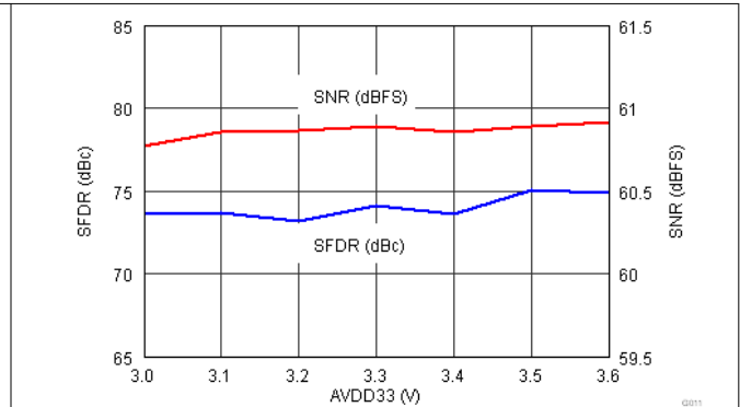
图 7-21. Performance Across AVDD33 (fin = 230 MHz)
