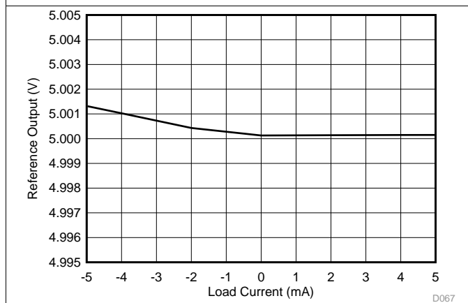
图 72. Internal Reference Voltage vs Load
