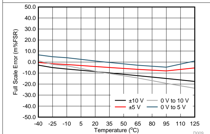
图 13. VOUT Full-Scale Error vs Temperature
