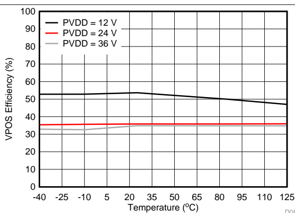
图 89. VOUT VPOS Efficiency vs Temperature
