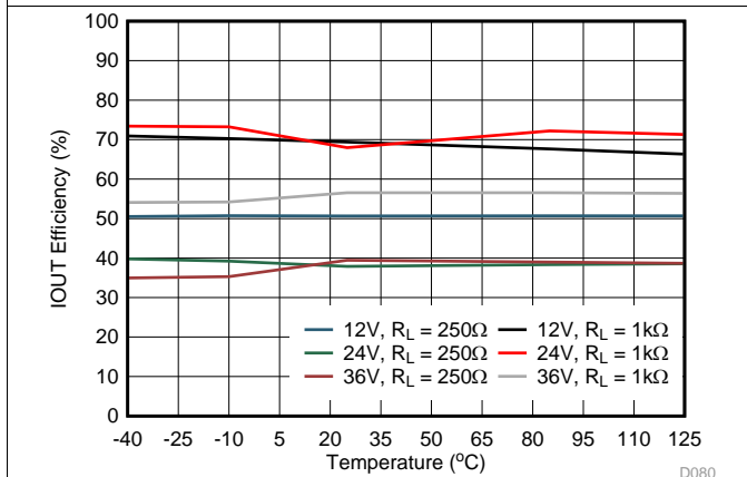
图 82. IOUT DC/DC Efficiency vs Temperature
