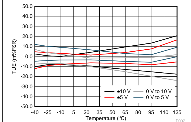
图 11. VOUT TUE vs Temperature
