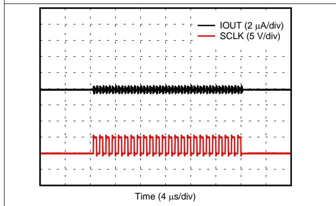
图 70. IOUT Digital Feed-Through
