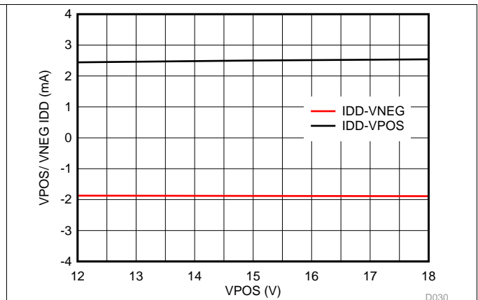
图 33. VOUT Quiescent Current vs VPOS (No Load)
