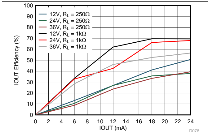
图 80. IOUT DC/DC Efficiency
