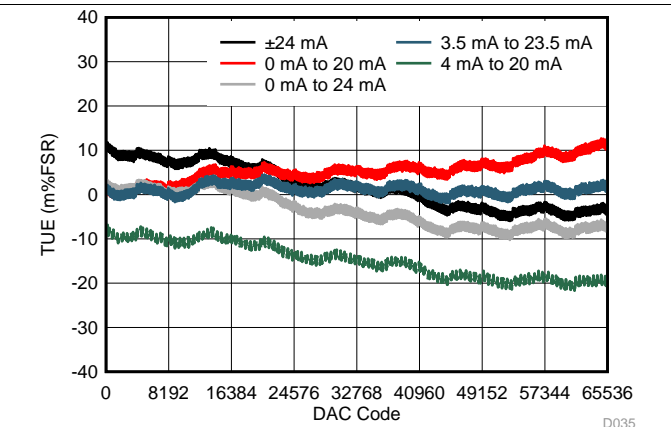
图 39. IOUT TUE vs Code (DC/DC Enabled)
