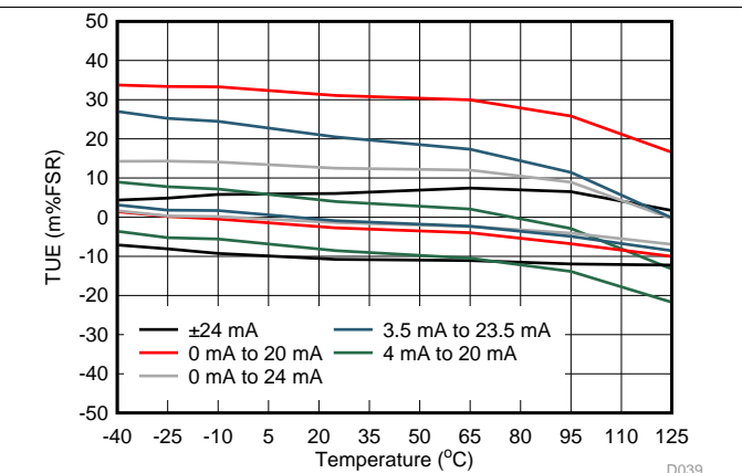
图 43. IOUT TUE vs Temperature
