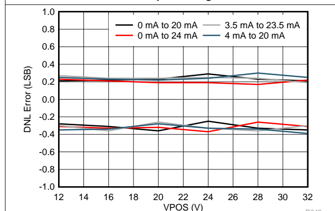
图 52. IOUT Unipolar Ranges DNL vs VPOS
