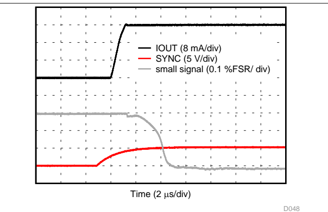
图 55. IOUT Settling Time, Rising Signal
