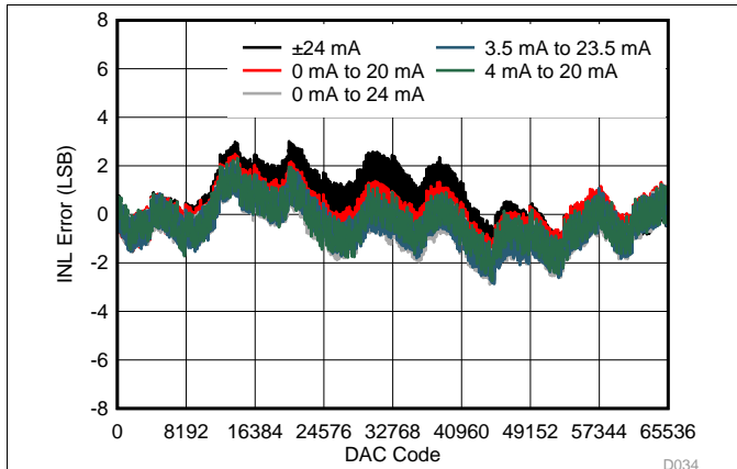
图 38. IOUT INL vs Code (DC/DC Disabled)
