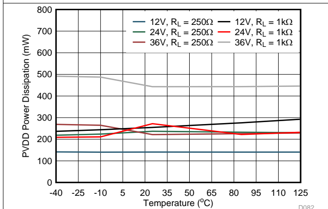
图 84. IOUT Power Dissipation vs Temperature
