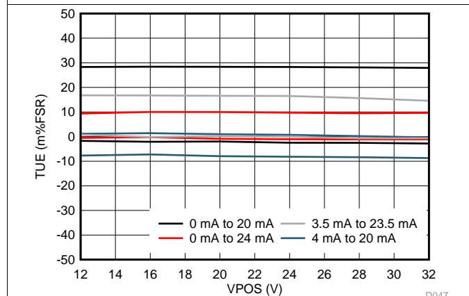
图 54. IOUT Unipolar Ranges TUE vs VPOS
