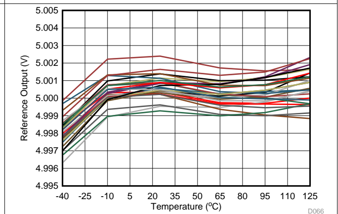
图 71. Internal Reference Voltage vs Temperature
