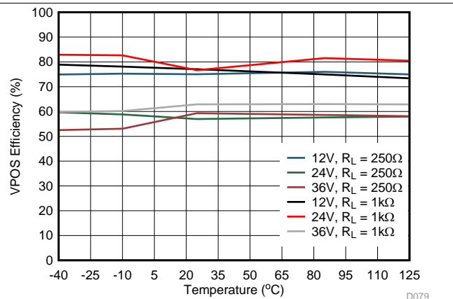
图 81. VPOS Efficiency vs Temperature
