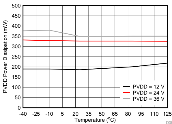
图 91. VOUT Power Dissipation vs Temperature
