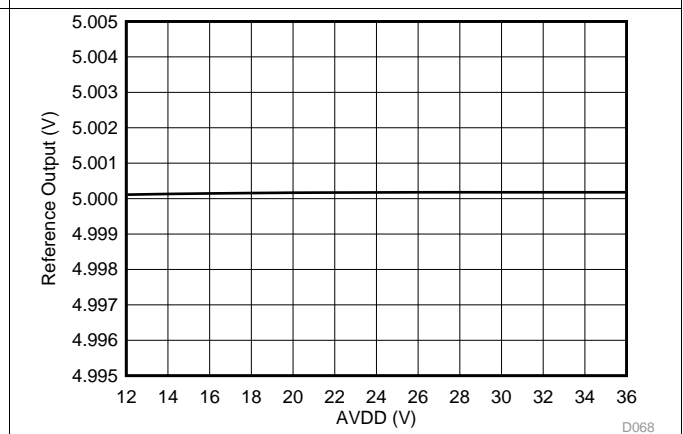
图 73. Internal Reference Voltage vs AVDD
