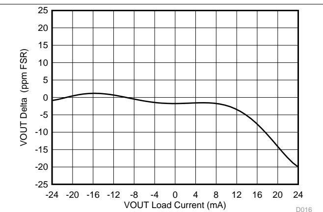
图 20. VOUT Load Regulation (SCLM = 11)
