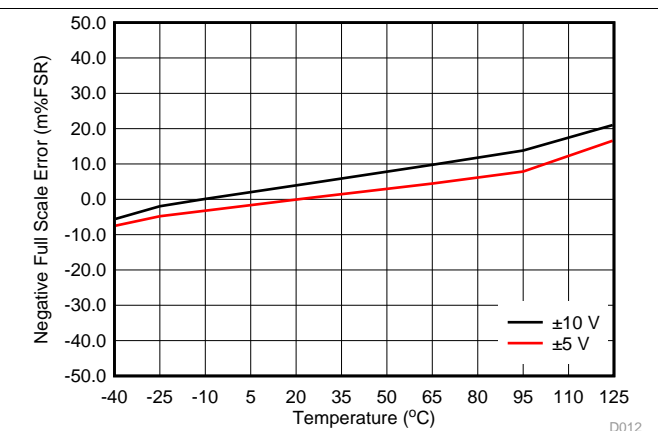
图 16. VOUT Negative Full-Scale Error vs Temperature
