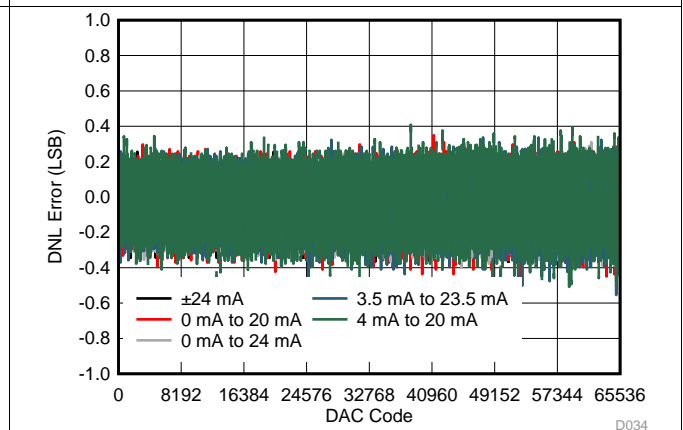
图 37. IOUT DNL vs Code (DC/DC Disabled)
