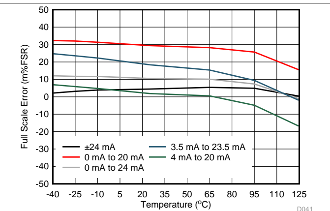
图 45. IOOUT Full-Scale Error vs Temperature
