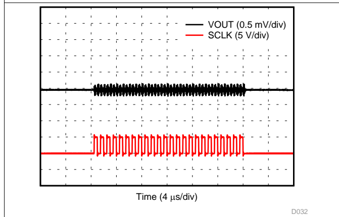
图 34. VOUT Digital Feedthrough
