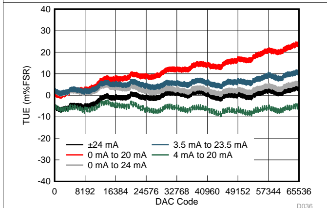
图 40. IOUT TUE vs Code (DC/DC Enabled)
