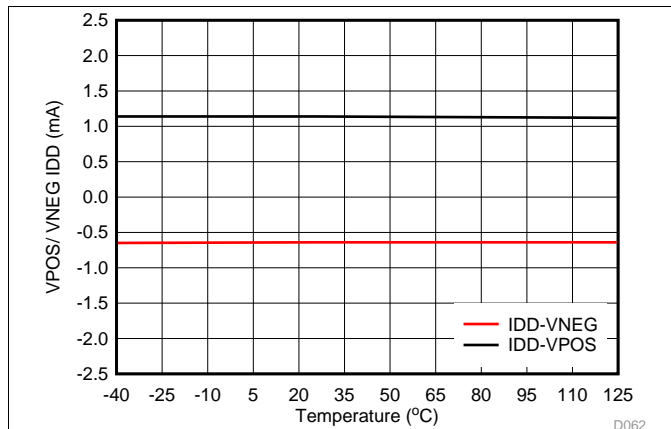
图 68. IOUT Quiescent Current vs Temperature
