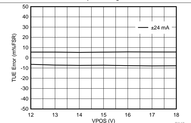
图 53. IOUT Bipolar Range TUE vs VPOS
