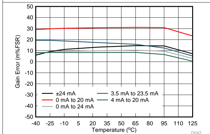
图 46. IOOUT Gain Error vs Temperature
