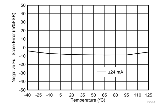
图 48. IOOUT Negative Full-Scale Error vs Temperature
