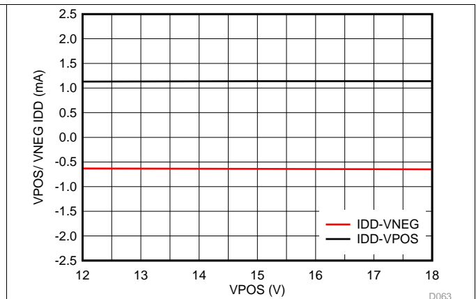
图 69. IOUT Quiescent Current vs VPOS
