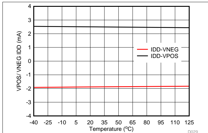
图 32. VOUT Quiescent Current vs Temperature (No Load)
