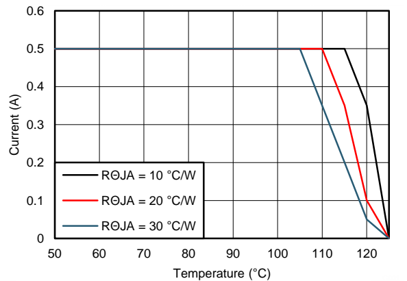
Figure 82. Derating Curve
