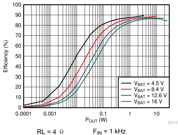
RL = 4 \Omega F_{\text{IN}} = 1 \text{ kHz} 图 6-13. Efficiency vs Output Power
