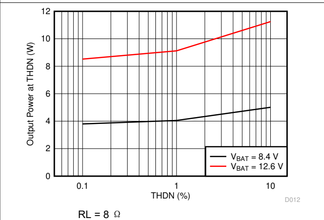
图 6-12. Max Output Power vs THD+N
