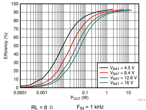
RL = 8 \Omega F_{\text{IN}} = 1 \text{ kHz} 图 6-14. Efficiency vs Output Power
