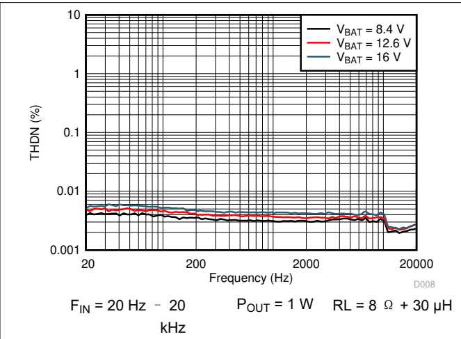
图 6-8. THD+N vs Frequency
